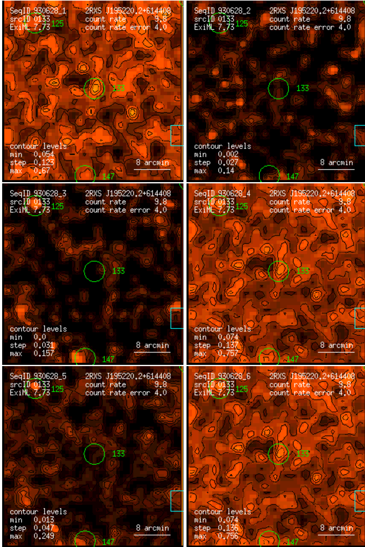
Figure 133: RASS 930628: detection 0133: band rate images, Gaussian filter: (1) PSPC channels 11 – 41, (2) 52 – 90, (3) 91 – 201, (4) 11 – 235, (5) 52 – 201, (6) 11 – 201. Broad band rates in counts/ks. Band rate contour levels in counts/ks/arcmin 2 .
