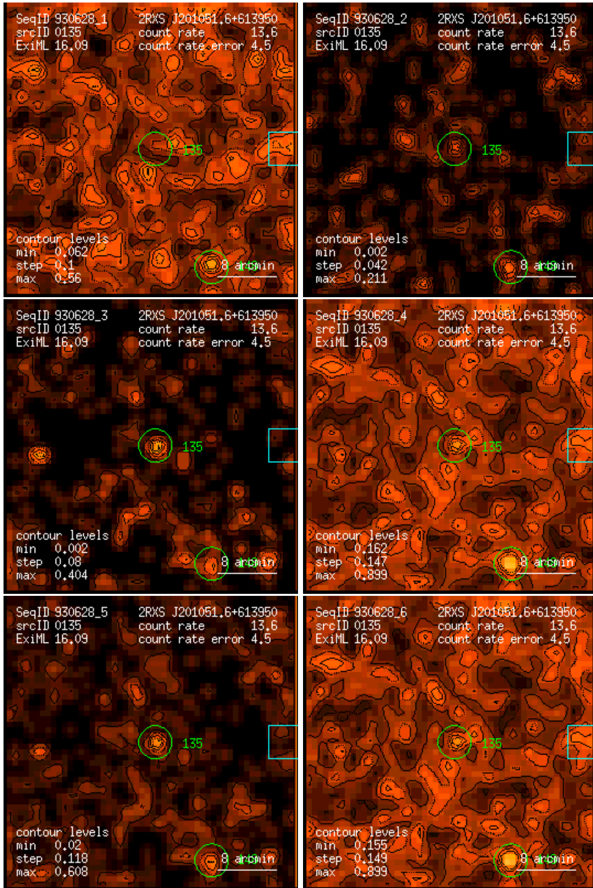
Figure 135: RASS 930628: detection 0135: band rate images, Gaussian filter: (1) PSPC channels 11 – 41, (2) 52 – 90, (3) 91 – 201, (4) 11 – 235, (5) 52 – 201, (6) 11 – 201. Broad band rates in counts/ks. Band rate contour levels in counts/ks/arcmin 2 .
