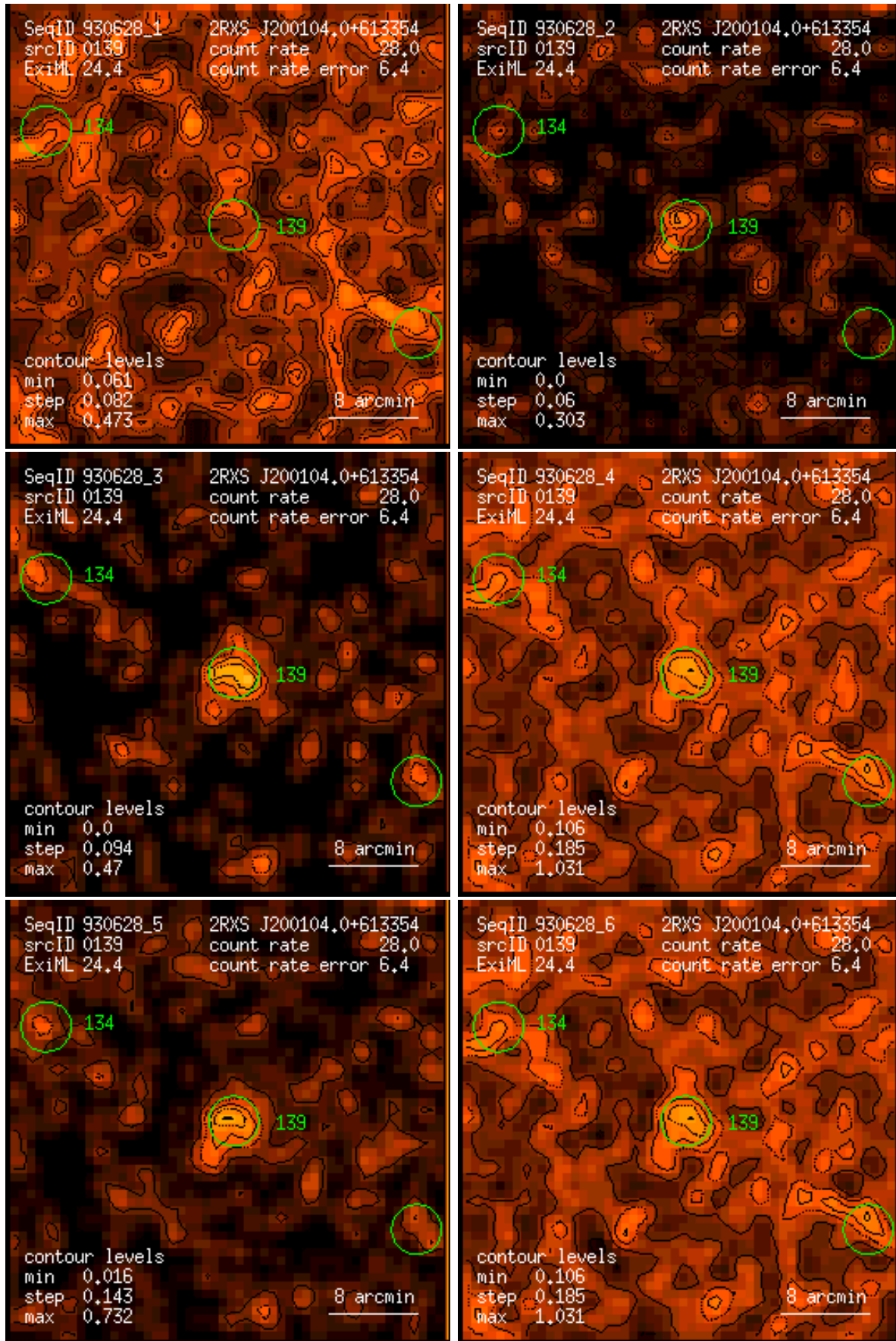
Figure 139: RASS 930628: detection 0139: band rate images, Gaussian filter: (1) PSPC channels 11 – 41, (2) 52 – 90, (3) 91 – 201, (4) 11 – 235, (5) 52 – 201, (6) 11 – 201. Broad band rates in counts/ks. Band rate contour levels in counts/ks/arcmin 2 .
