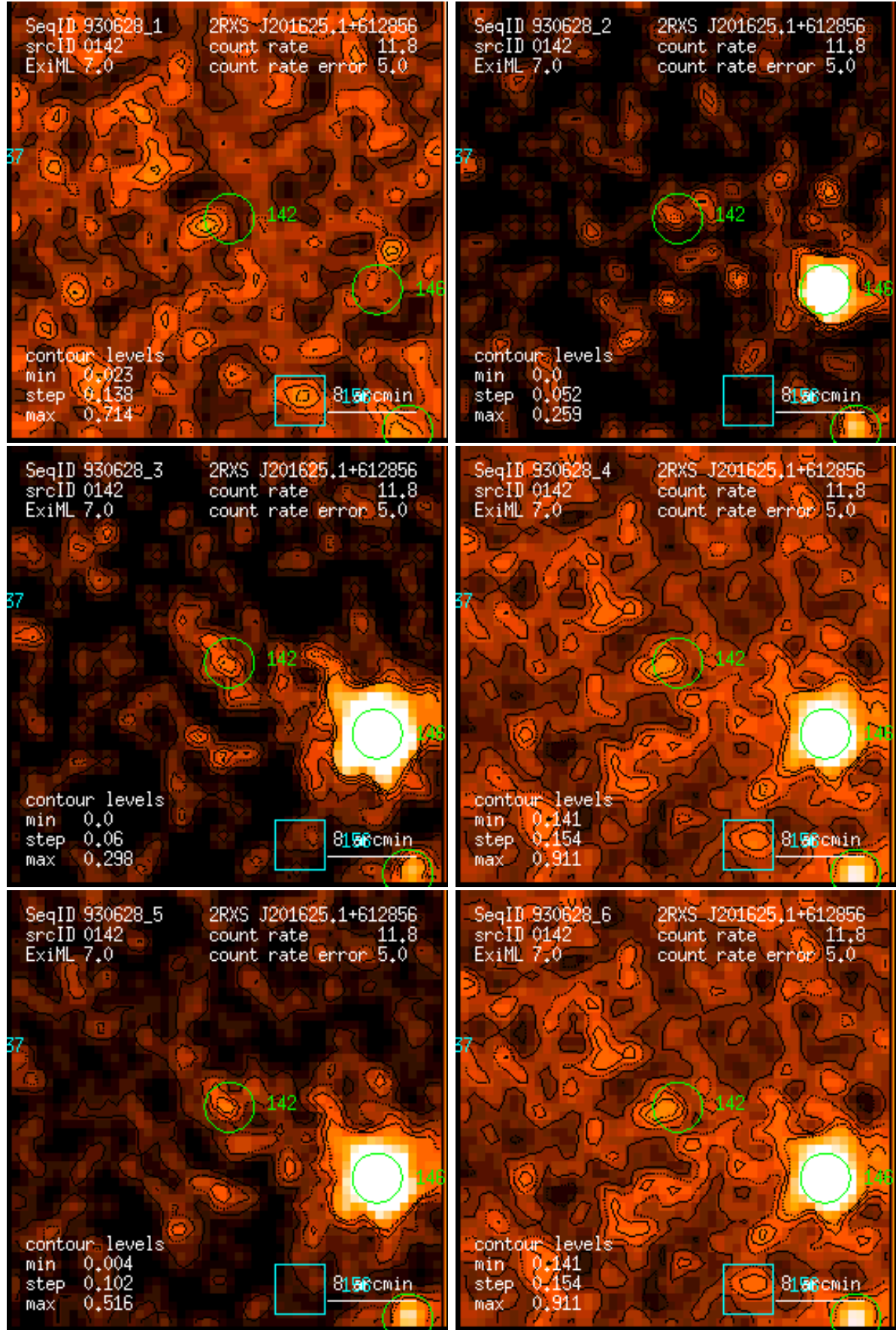
Figure 142: RASS 930628: detection 0142: band rate images, Gaussian filter: (1) PSPC channels 11 – 41, (2) 52 – 90, (3) 91 – 201, (4) 11 – 235, (5) 52 – 201, (6) 11 – 201. Broad band rates in counts/ks. Band rate contour levels in counts/ks/arcmin 2 .
