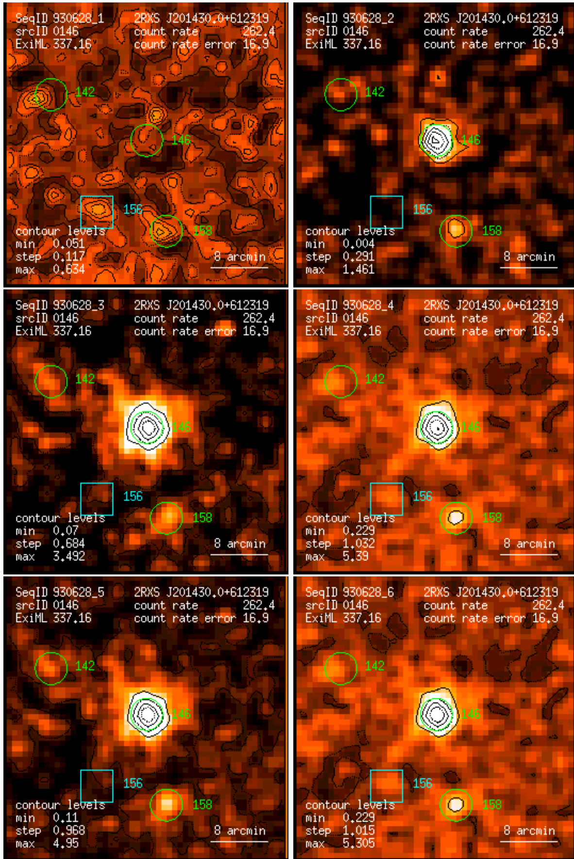
Figure 146: RASS 930628: detection 0146: band rate images, Gaussian filter: (1) PSPC channels 11 – 41, (2) 52 – 90, (3) 91 – 201, (4) 11 – 235, (5) 52 – 201, (6) 11 – 201. Broad band rates in counts/ks. Band rate contour levels in counts/ks/arcmin 2 .
