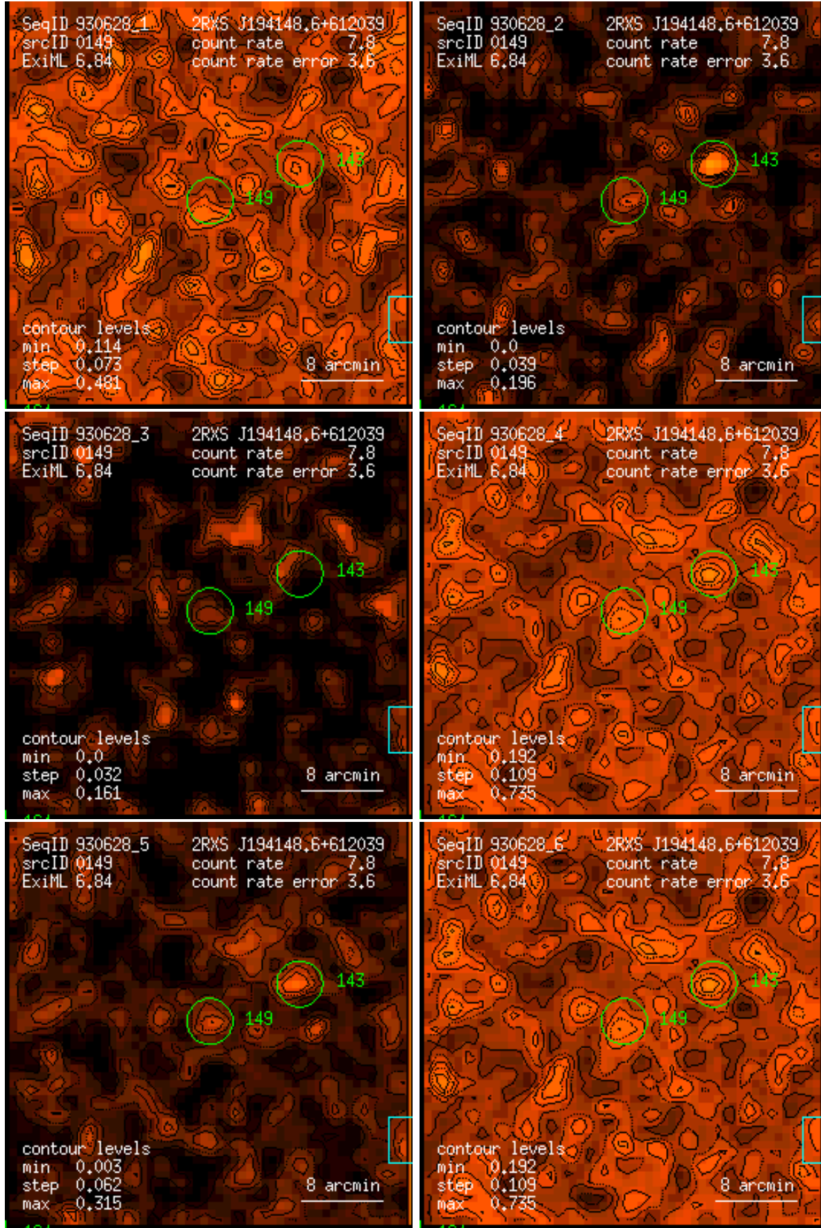
Figure 149: RASS 930628: detection 0149: band rate images, Gaussian filter: (1) PSPC channels 11 – 41, (2) 52 – 90, (3) 91 – 201, (4) 11 – 235, (5) 52 – 201, (6) 11 – 201. Broad band rates in counts/ks. Band rate contour levels in counts/ks/arcmin 2 .
