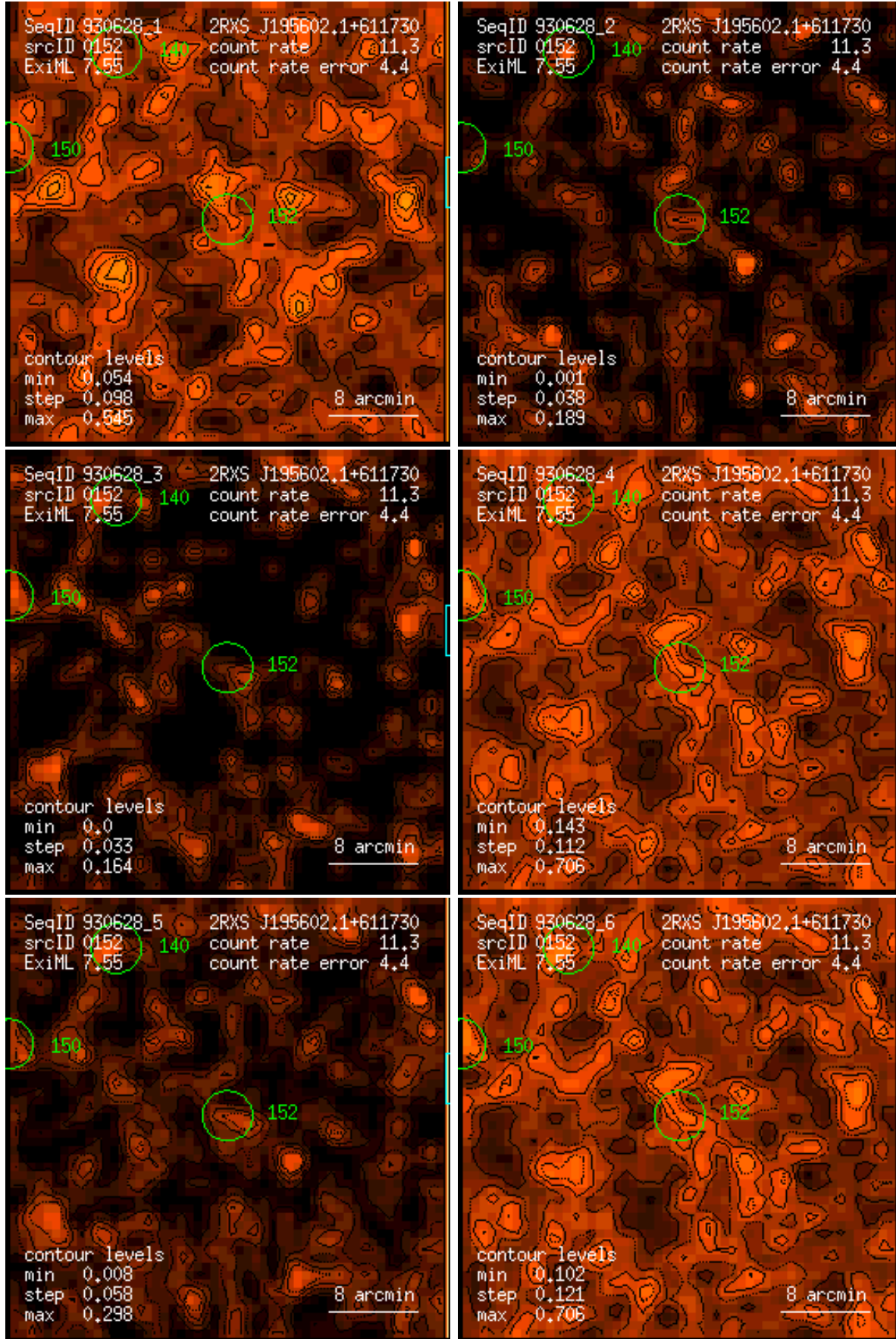
Figure 152: RASS 930628: detection 0152: band rate images, Gaussian filter: (1) PSPC channels 11 – 41, (2) 52 – 90, (3) 91 – 201, (4) 11 – 235, (5) 52 – 201, (6) 11 – 201. Broad band rates in counts/ks. Band rate contour levels in counts/ks/arcmin 2 .
