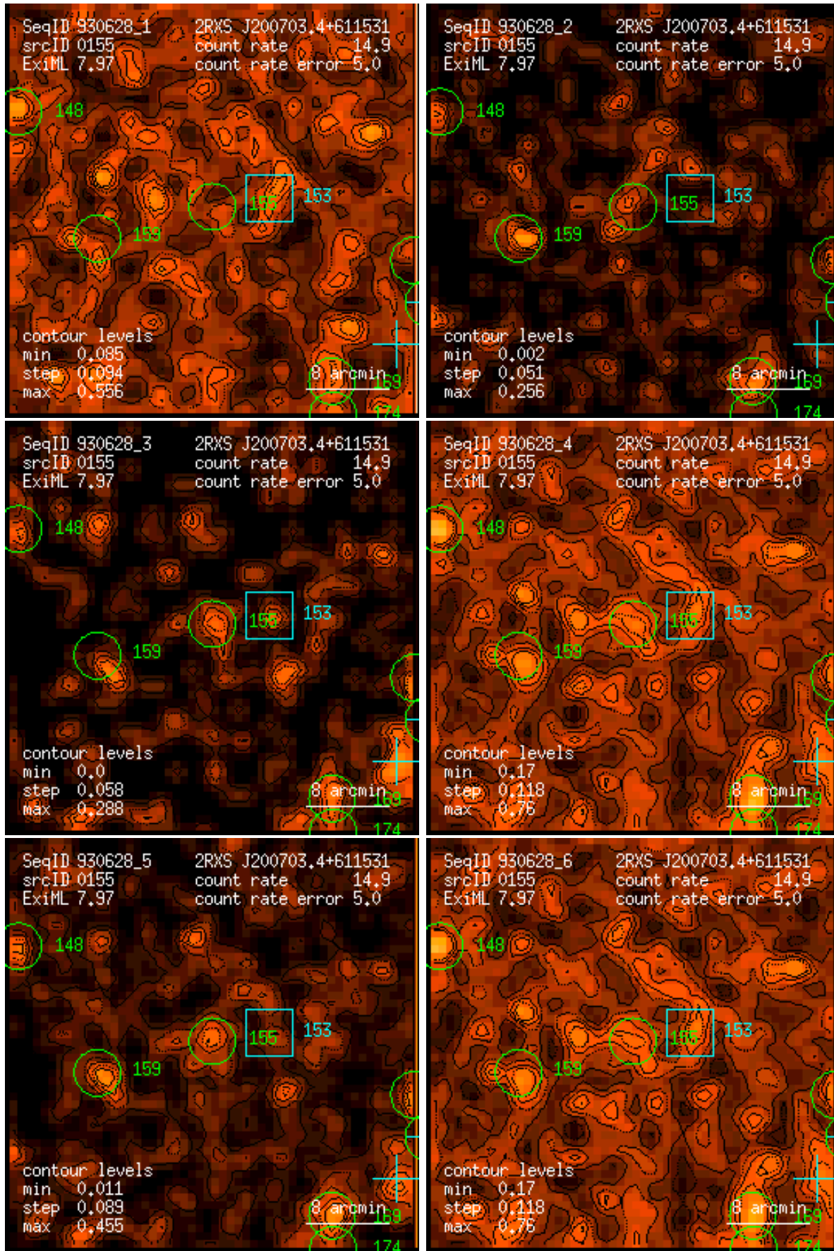
Figure 155: RASS 930628: detection 0155: band rate images, Gaussian filter: (1) PSPC channels 11 – 41, (2) 52 – 90, (3) 91 – 201, (4) 11 – 235, (5) 52 – 201, (6) 11 – 201. Broad band rates in counts/ks. Band rate contour levels in counts/ks/arcmin 2 .
