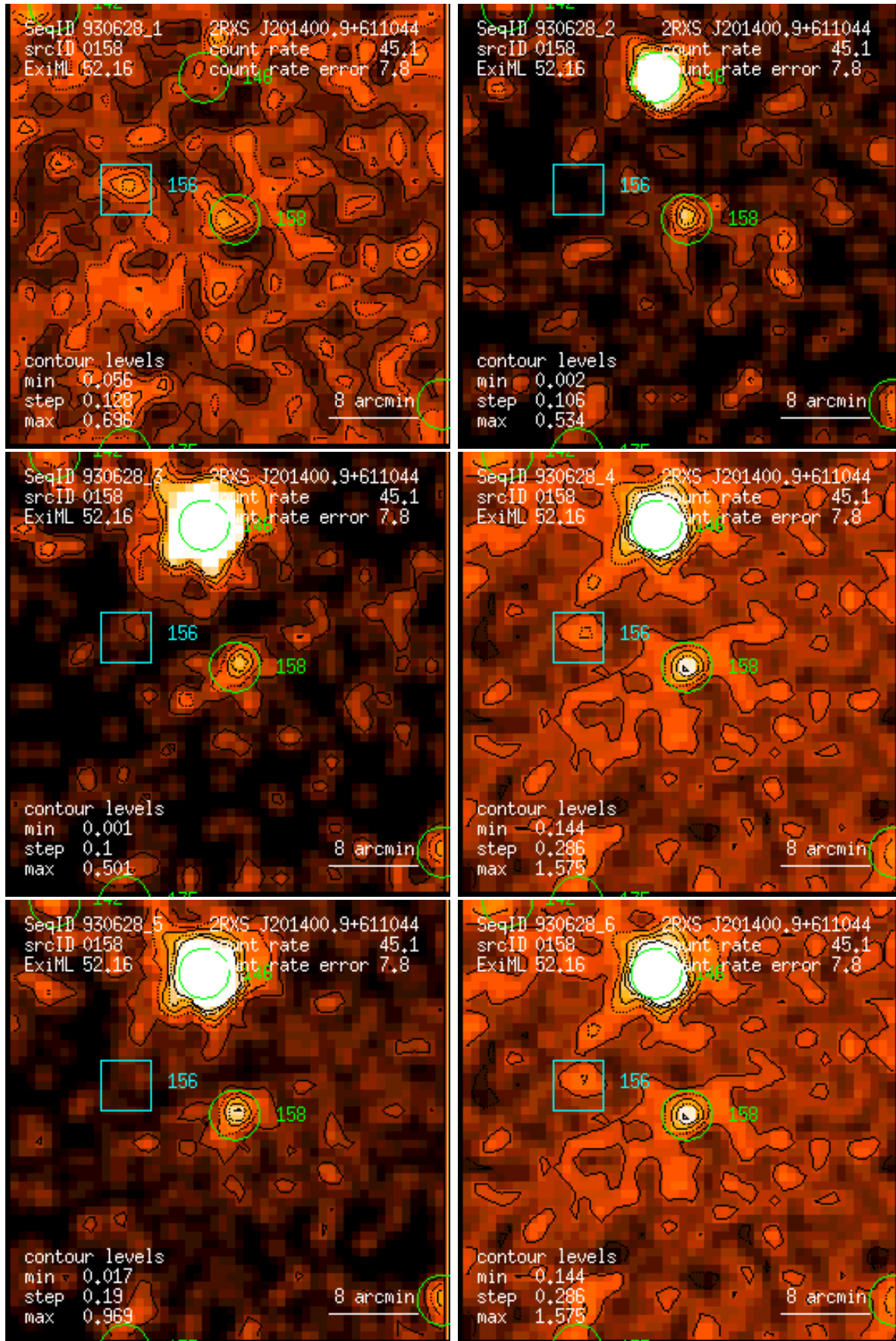
Figure 158: RASS 930628: detection 0158: band rate images, Gaussian filter: (1) PSPC channels 11 – 41, (2) 52 – 90, (3) 91 – 201, (4) 11 – 235, (5) 52 – 201, (6) 11 – 201. Broad band rates in counts/ks. Band rate contour levels in counts/ks/arcmin 2 .
