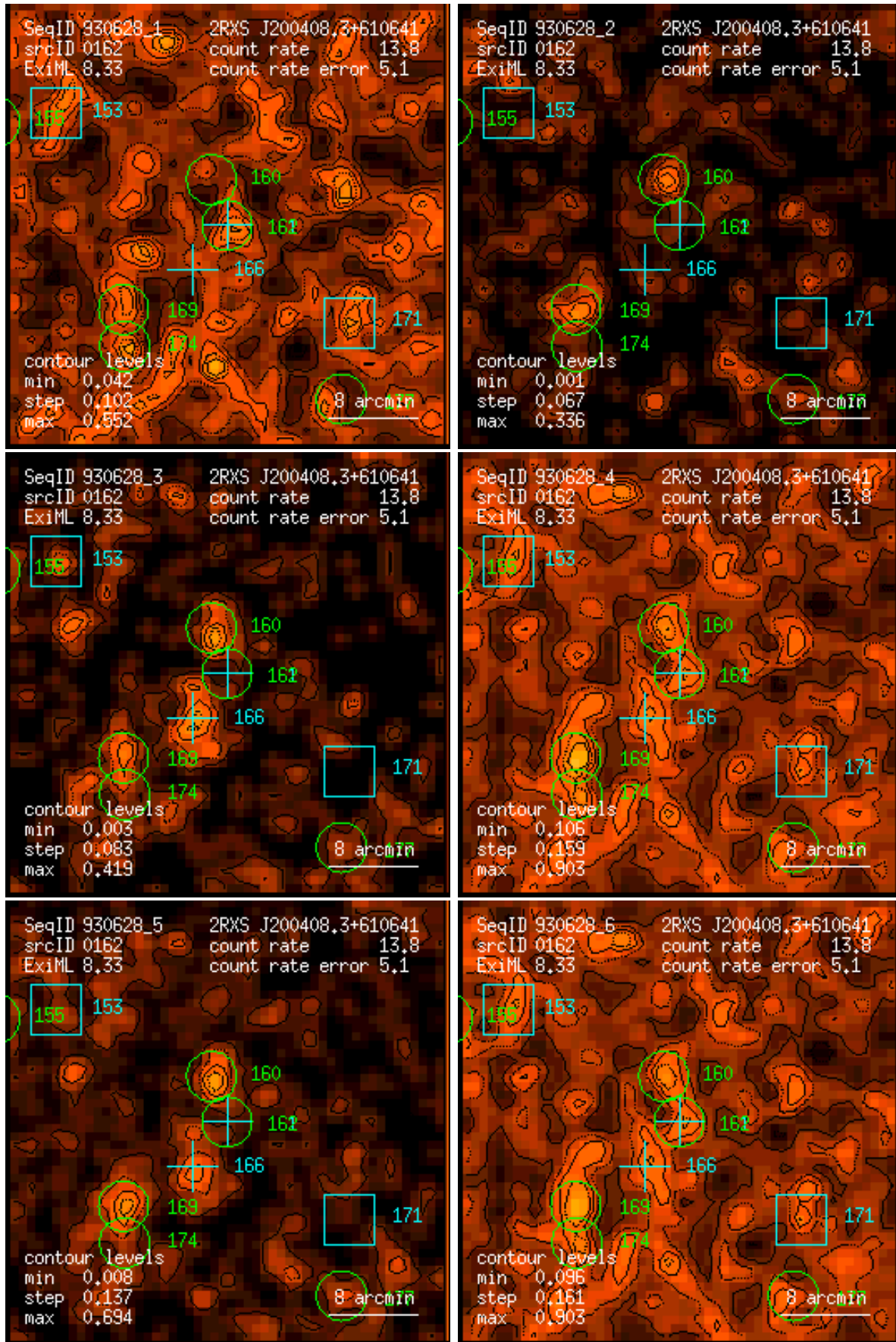
Figure 162: RASS 930628: detection 0162: band rate images, Gaussian filter: (1) PSPC channels 11 – 41, (2) 52 – 90, (3) 91 – 201, (4) 11 – 235, (5) 52 – 201, (6) 11 – 201. Broad band rates in counts/ks. Band rate contour levels in counts/ks/arcmin 2 .
