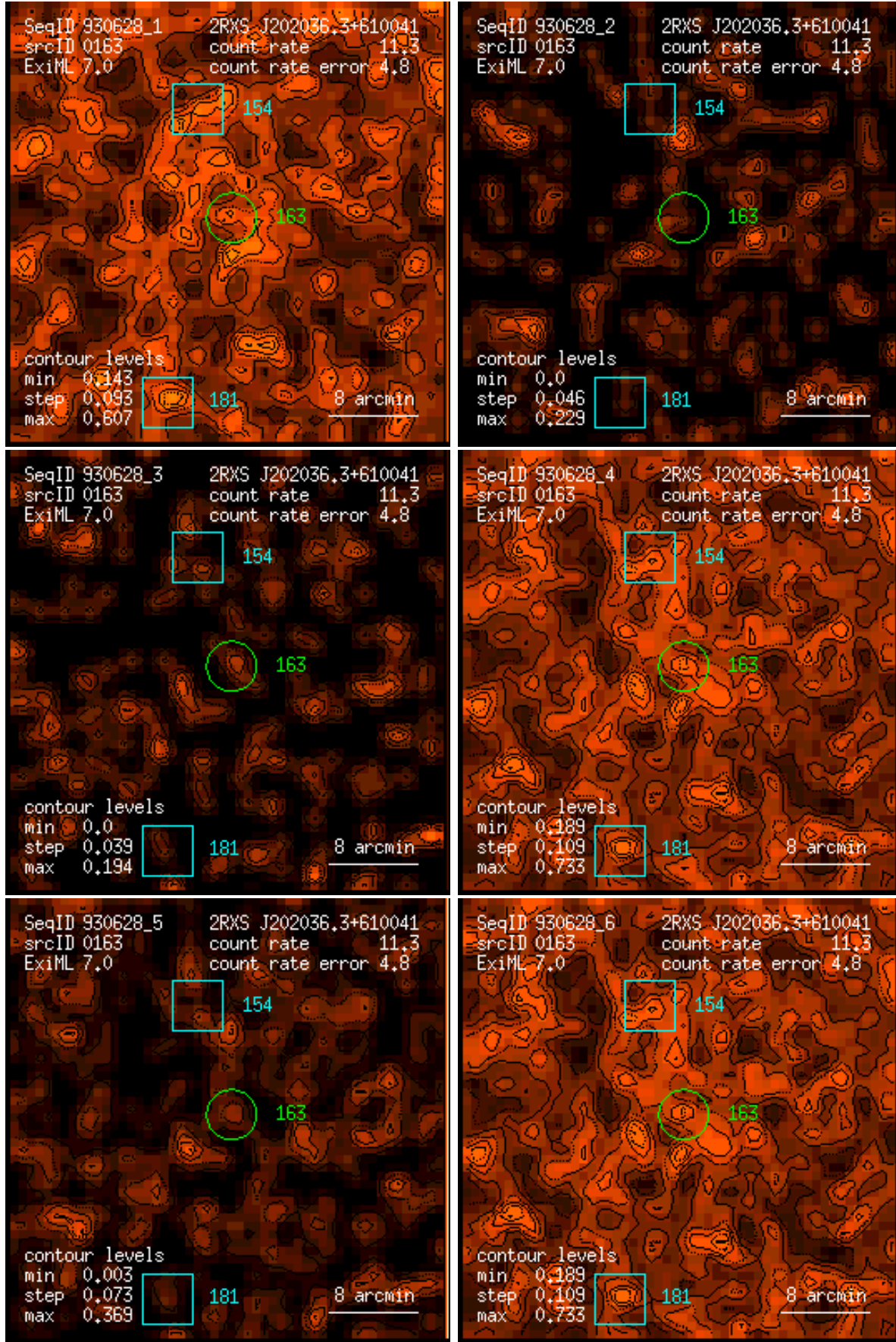
Figure 163: RASS 930628: detection 0163: band rate images, Gaussian filter: (1) PSPC channels 11 – 41, (2) 52 – 90, (3) 91 – 201, (4) 11 – 235, (5) 52 – 201, (6) 11 – 201. Broad band rates in counts/ks. Band rate contour levels in counts/ks/arcmin 2 .
