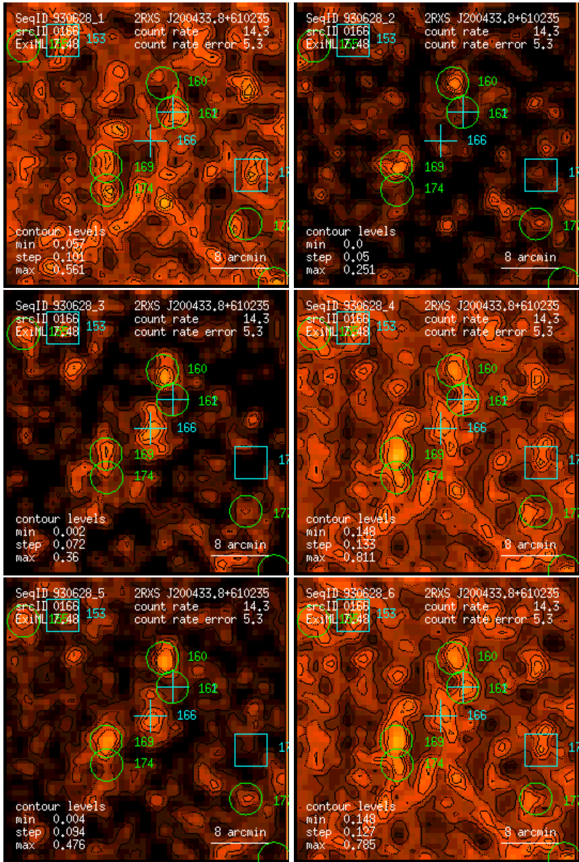
Figure 166: RASS 930628: detection 0166: band rate images, Gaussian filter: (1) PSPC channels 11 – 41, (2) 52 – 90, (3) 91 – 201, (4) 11 – 235, (5) 52 – 201, (6) 11 – 201. Broad band rates in counts/ks. Band rate contour levels in counts/ks/arcmin 2 .
