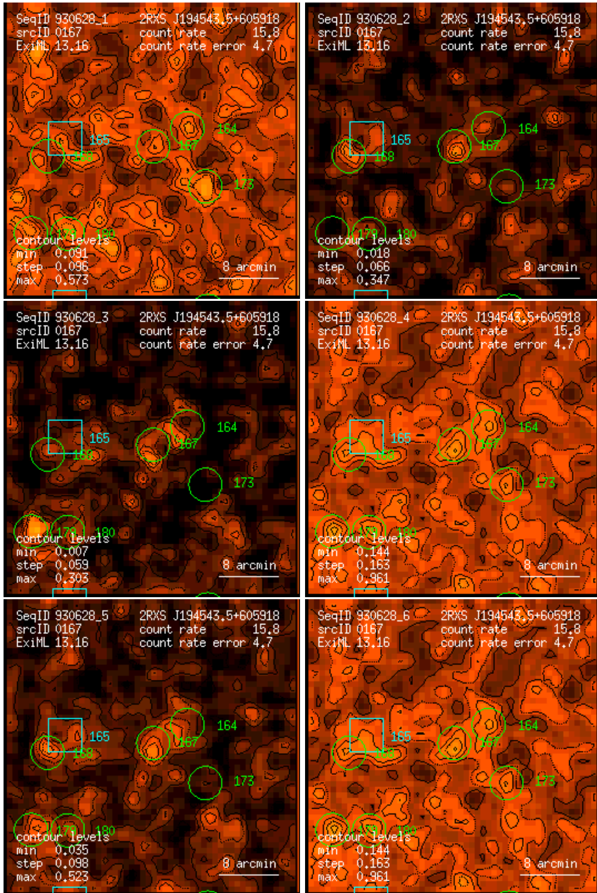
Figure 167: RASS 930628: detection 0167: band rate images, Gaussian filter: (1) PSPC channels 11 – 41, (2) 52 – 90, (3) 91 – 201, (4) 11 – 235, (5) 52 – 201, (6) 11 – 201. Broad band rates in counts/ks. Band rate contour levels in counts/ks/arcmin 2 .
