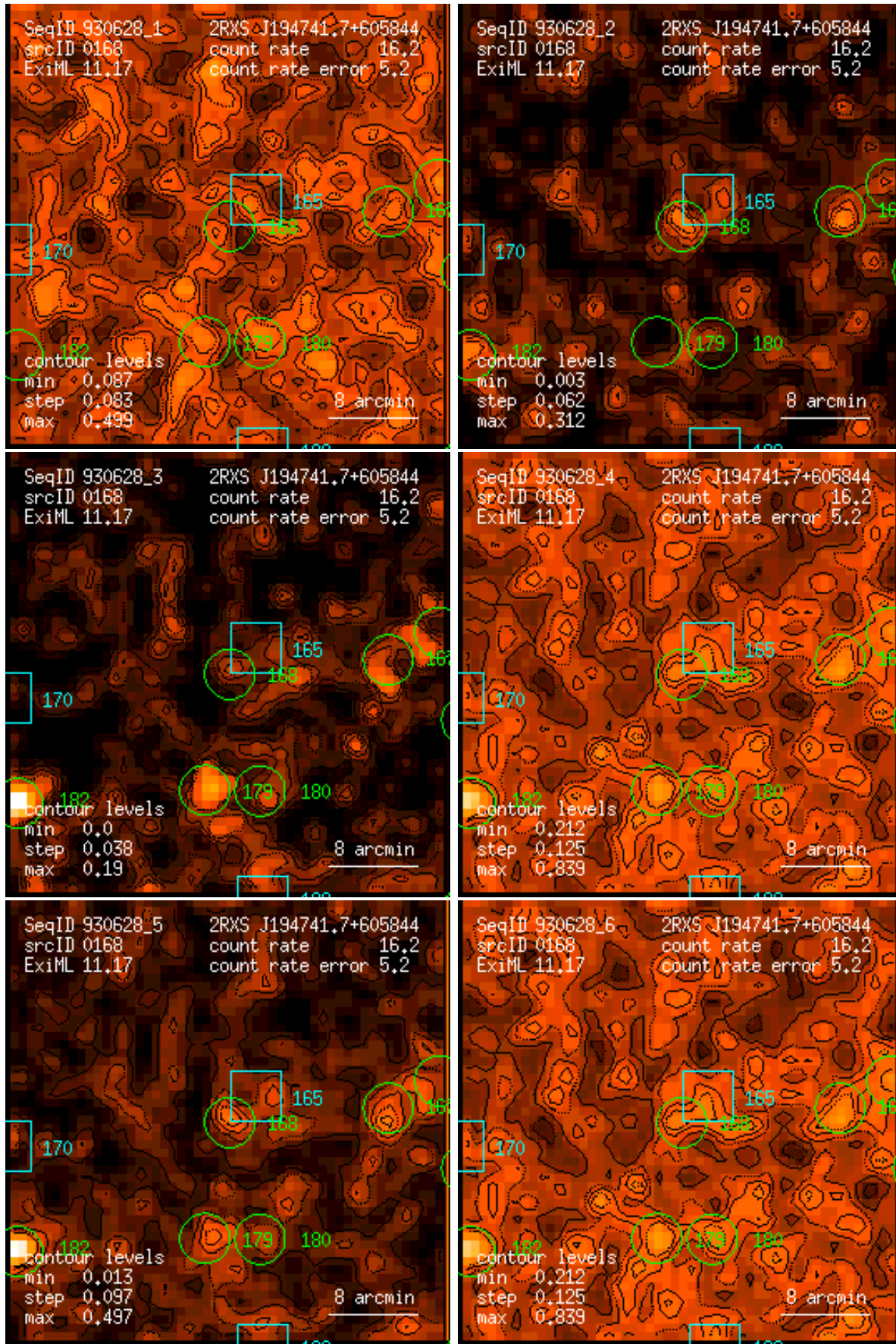
Figure 168: RASS 930628: detection 0168: band rate images, Gaussian filter: (1) PSPC channels 11 – 41, (2) 52 – 90, (3) 91 – 201, (4) 11 – 235, (5) 52 – 201, (6) 11 – 201. Broad band rates in counts/ks. Band rate contour levels in counts/ks/arcmin 2 .
