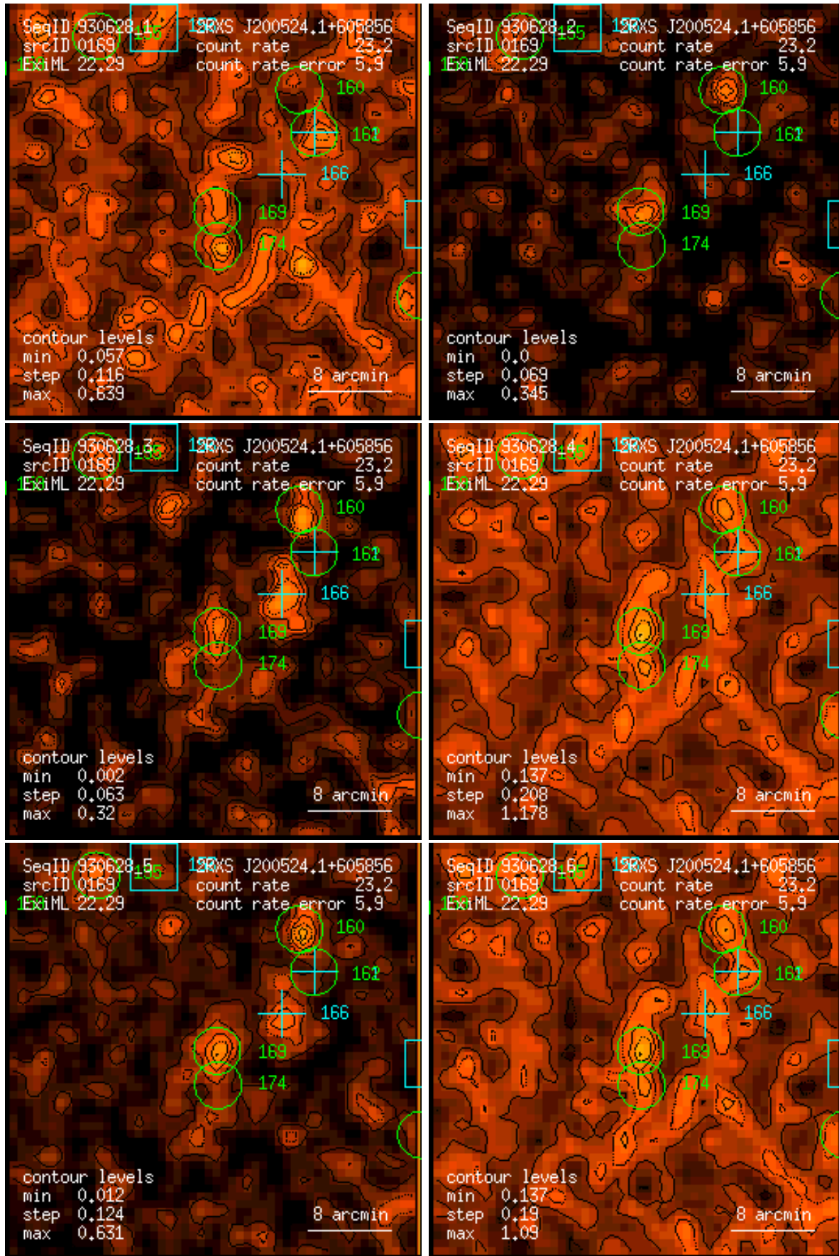
Figure 169: RASS 930628: detection 0169: band rate images, Gaussian filter: (1) PSPC channels 11 – 41, (2) 52 – 90, (3) 91 – 201, (4) 11 – 235, (5) 52 – 201, (6) 11 – 201. Broad band rates in counts/ks. Band rate contour levels in counts/ks/arcmin 2 .
