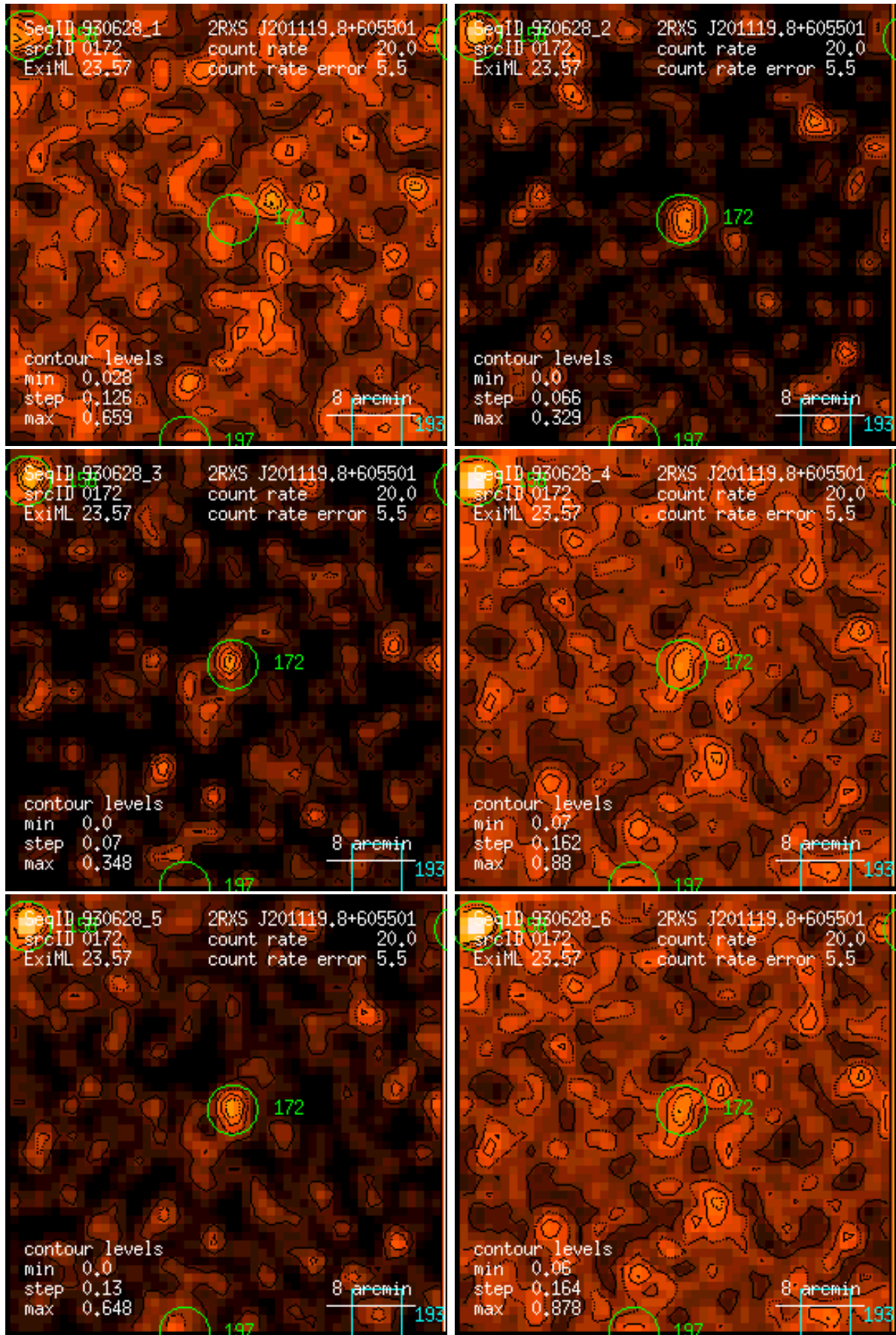
Figure 172: RASS 930628: detection 0172: band rate images, Gaussian filter: (1) PSPC channels 11 – 41, (2) 52 – 90, (3) 91 – 201, (4) 11 – 235, (5) 52 – 201, (6) 11 – 201. Broad band rates in counts/ks. Band rate contour levels in counts/ks/arcmin 2 .
