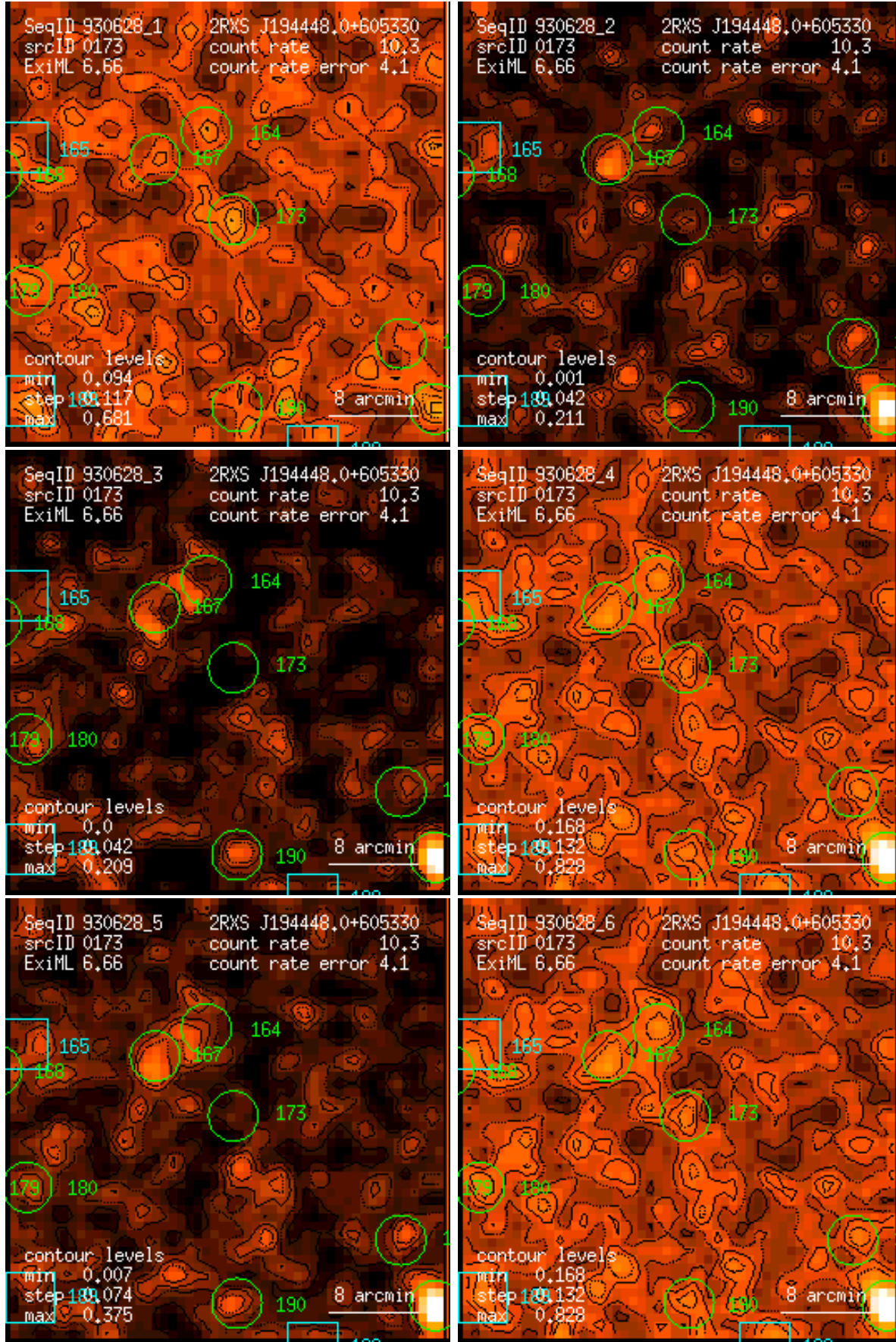
Figure 173: RASS 930628: detection 0173: band rate images, Gaussian filter: (1) PSPC channels 11 – 41, (2) 52 – 90, (3) 91 – 201, (4) 11 – 235, (5) 52 – 201, (6) 11 – 201. Broad band rates in counts/ks. Band rate contour levels in counts/ks/arcmin 2 .
