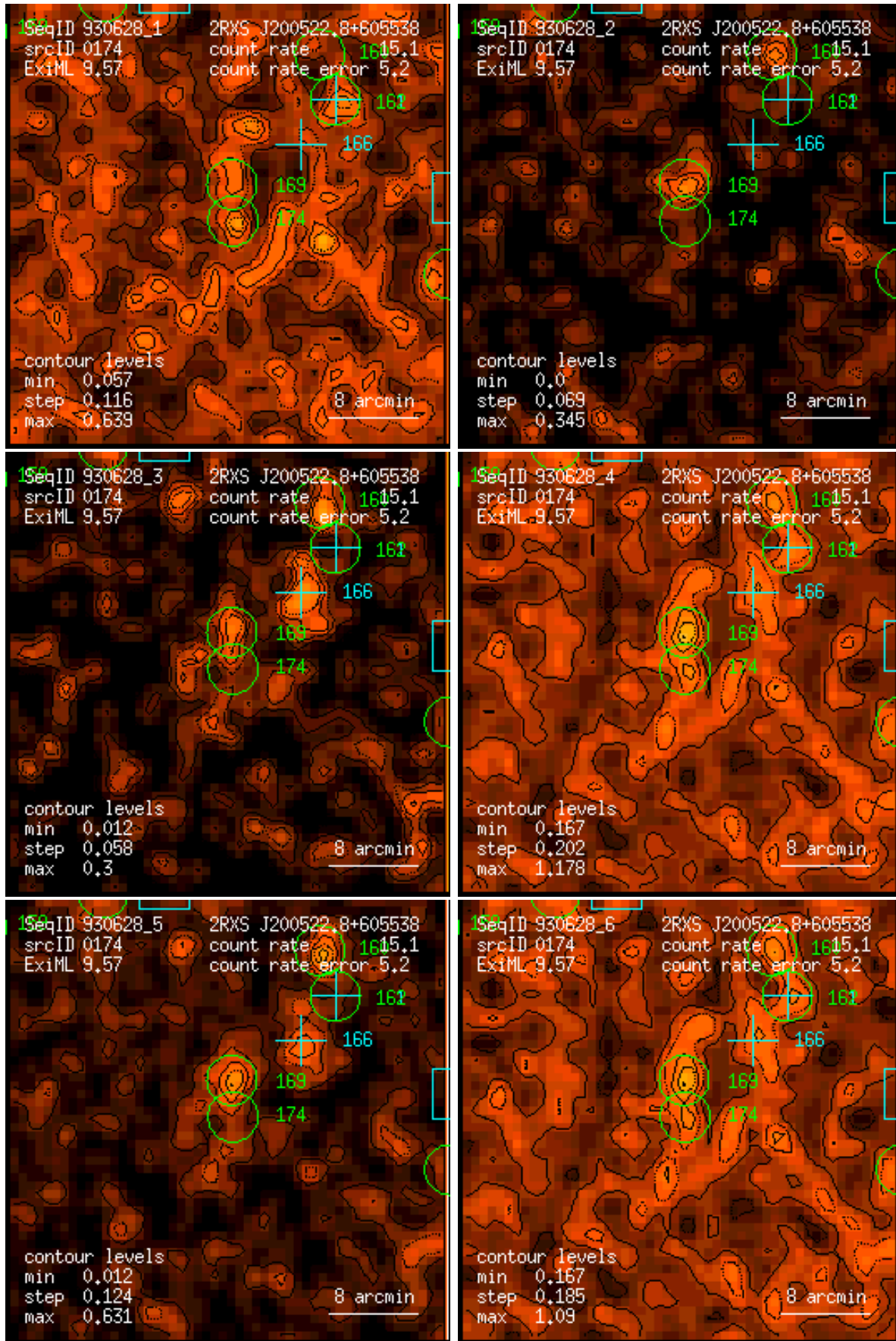
Figure 174: RASS 930628: detection 0174: band rate images, Gaussian filter: (1) PSPC channels 11 – 41, (2) 52 – 90, (3) 91 – 201, (4) 11 – 235, (5) 52 – 201, (6) 11 – 201. Broad band rates in counts/ks. Band rate contour levels in counts/ks/arcmin 2 .
