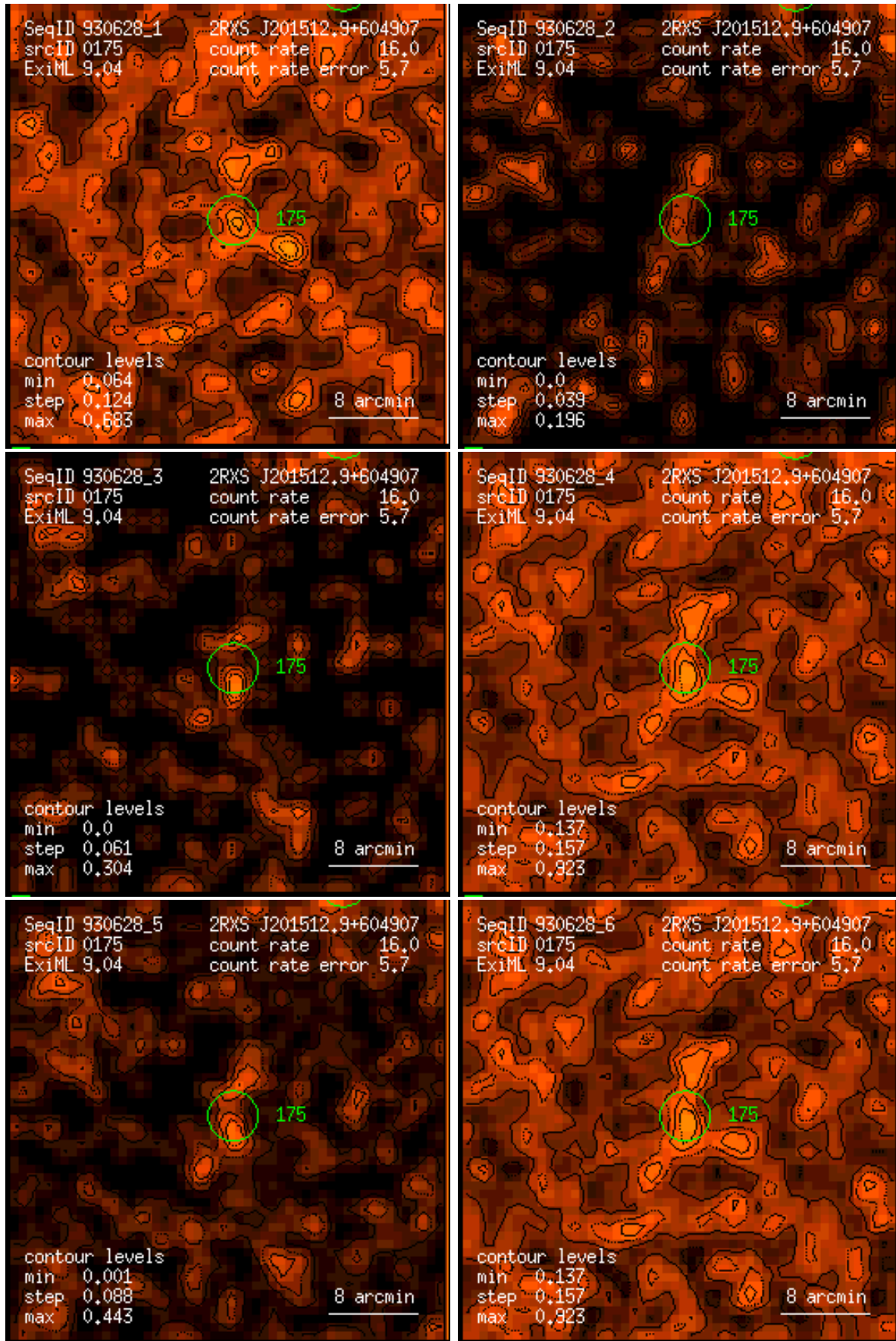
Figure 175: RASS 930628: detection 0175: band rate images, Gaussian filter: (1) PSPC channels 11 – 41, (2) 52 – 90, (3) 91 – 201, (4) 11 – 235, (5) 52 – 201, (6) 11 – 201. Broad band rates in counts/ks. Band rate contour levels in counts/ks/arcmin 2 .
