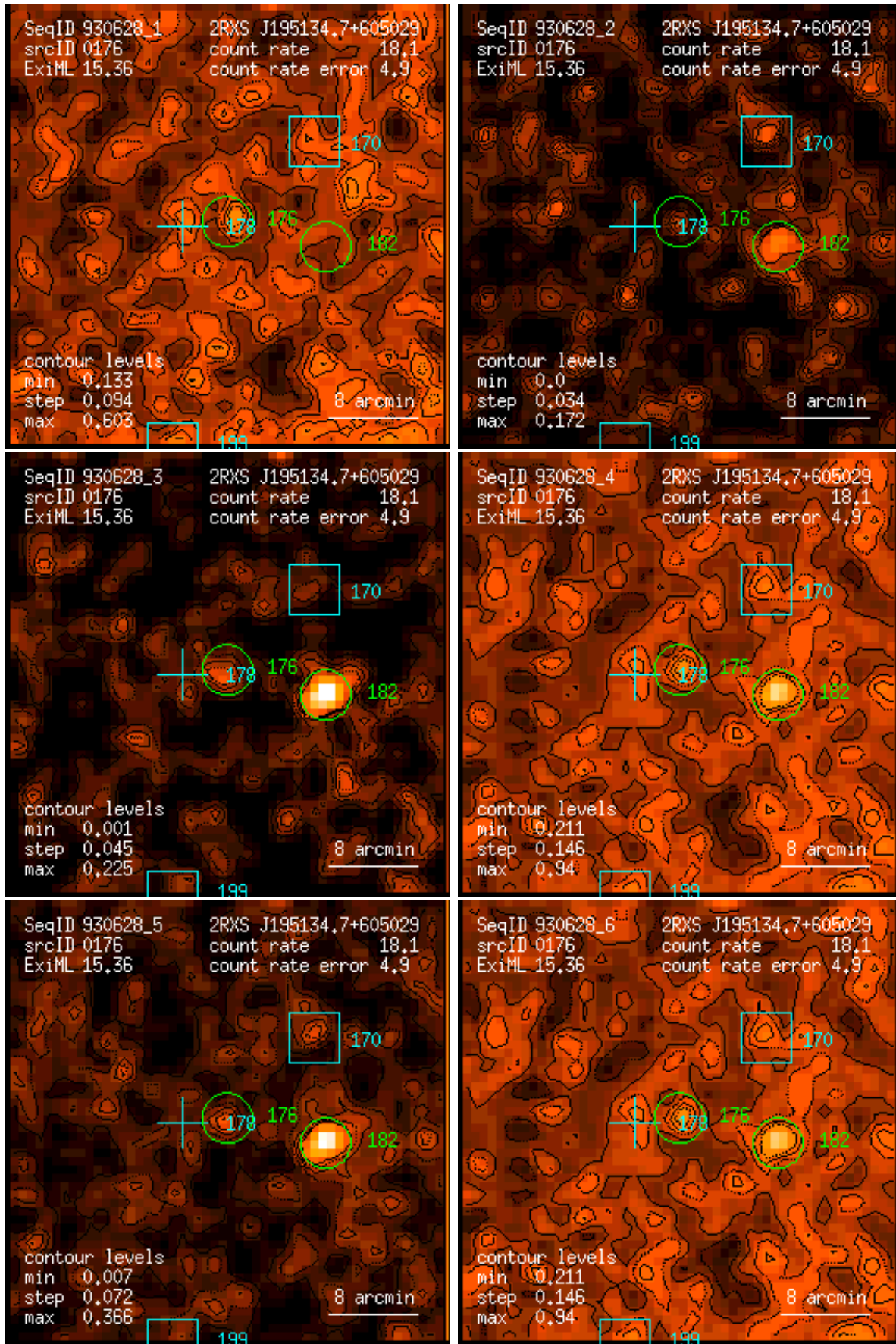
Figure 176: RASS 930628: detection 0176: band rate images, Gaussian filter: (1) PSPC channels 11 – 41, (2) 52 – 90, (3) 91 – 201, (4) 11 – 235, (5) 52 – 201, (6) 11 – 201. Broad band rates in counts/ks. Band rate contour levels in counts/ks/arcmin 2 .
