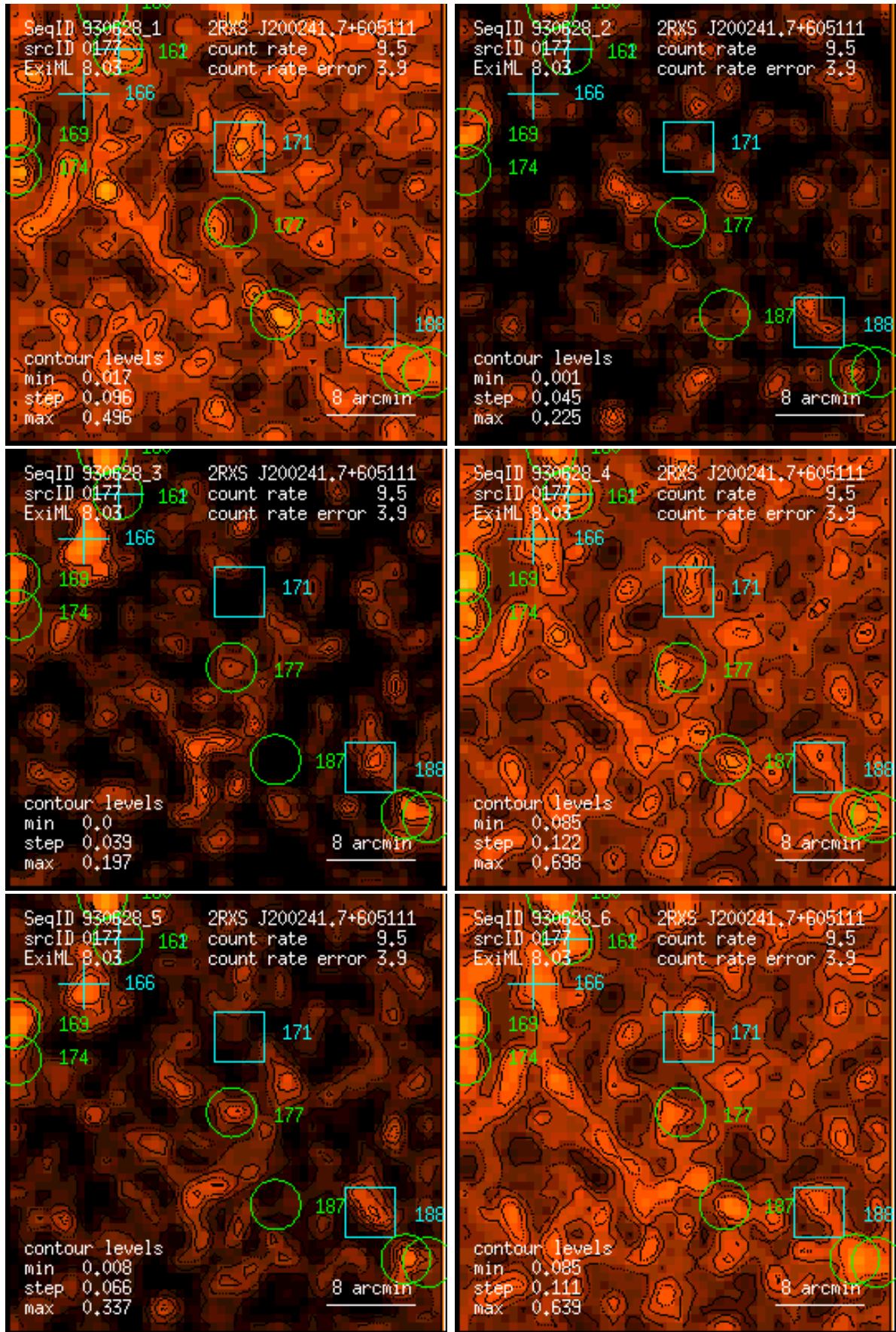
Figure 177: RASS 930628: detection 0177: band rate images, Gaussian filter: (1) PSPC channels 11 – 41, (2) 52 – 90, (3) 91 – 201, (4) 11 – 235, (5) 52 – 201, (6) 11 – 201. Broad band rates in counts/ks. Band rate contour levels in counts/ks/arcmin 2 .
