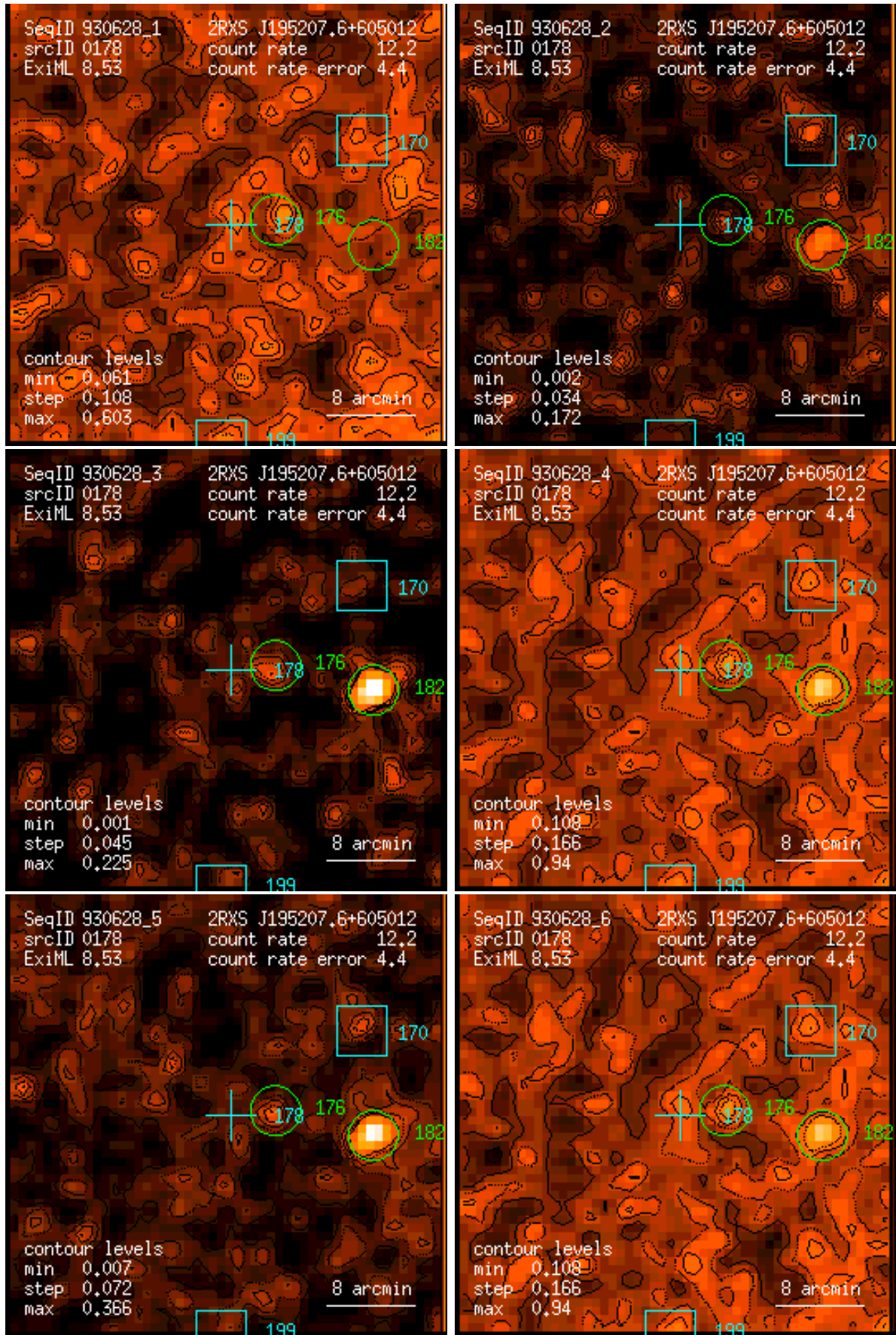
Figure 178: RASS 930628: detection 0178: band rate images, Gaussian filter: (1) PSPC channels 11 – 41, (2) 52 – 90, (3) 91 – 201, (4) 11 – 235, (5) 52 – 201, (6) 11 – 201. Broad band rates in counts/ks. Band rate contour levels in counts/ks/arcmin 2 .
