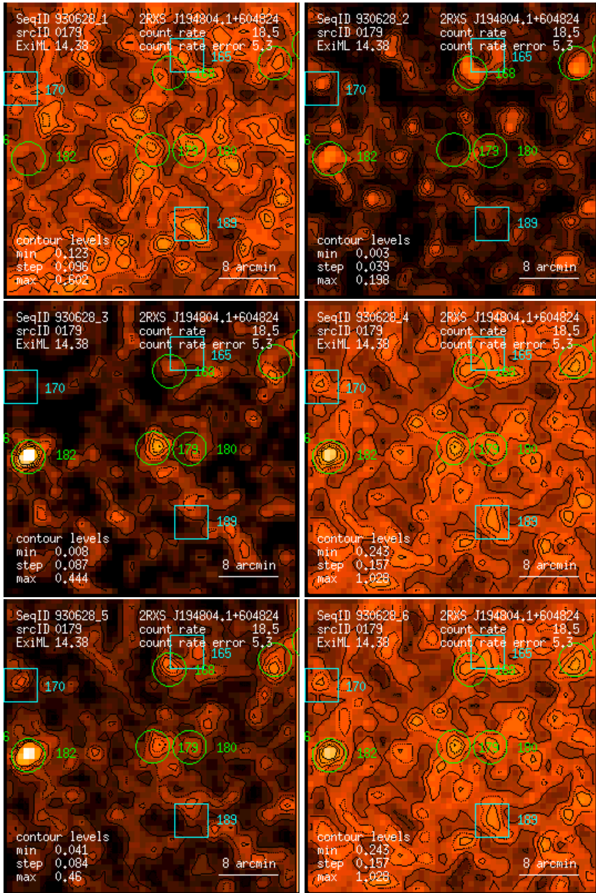
Figure 179: RASS 930628: detection 0179: band rate images, Gaussian filter: (1) PSPC channels 11 – 41, (2) 52 – 90, (3) 91 – 201, (4) 11 – 235, (5) 52 – 201, (6) 11 – 201. Broad band rates in counts/ks. Band rate contour levels in counts/ks/arcmin 2 .
