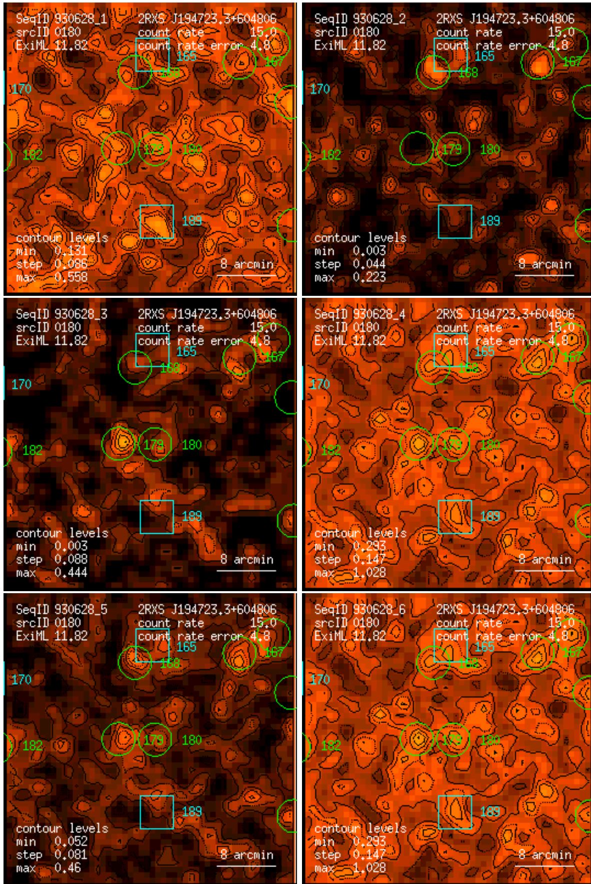
Figure 180: RASS 930628: detection 0180: band rate images, Gaussian filter: (1) PSPC channels 11 – 41, (2) 52 – 90, (3) 91 – 201, (4) 11 – 235, (5) 52 – 201, (6) 11 – 201. Broad band rates in counts/ks. Band rate contour levels in counts/ks/arcmin 2 .
