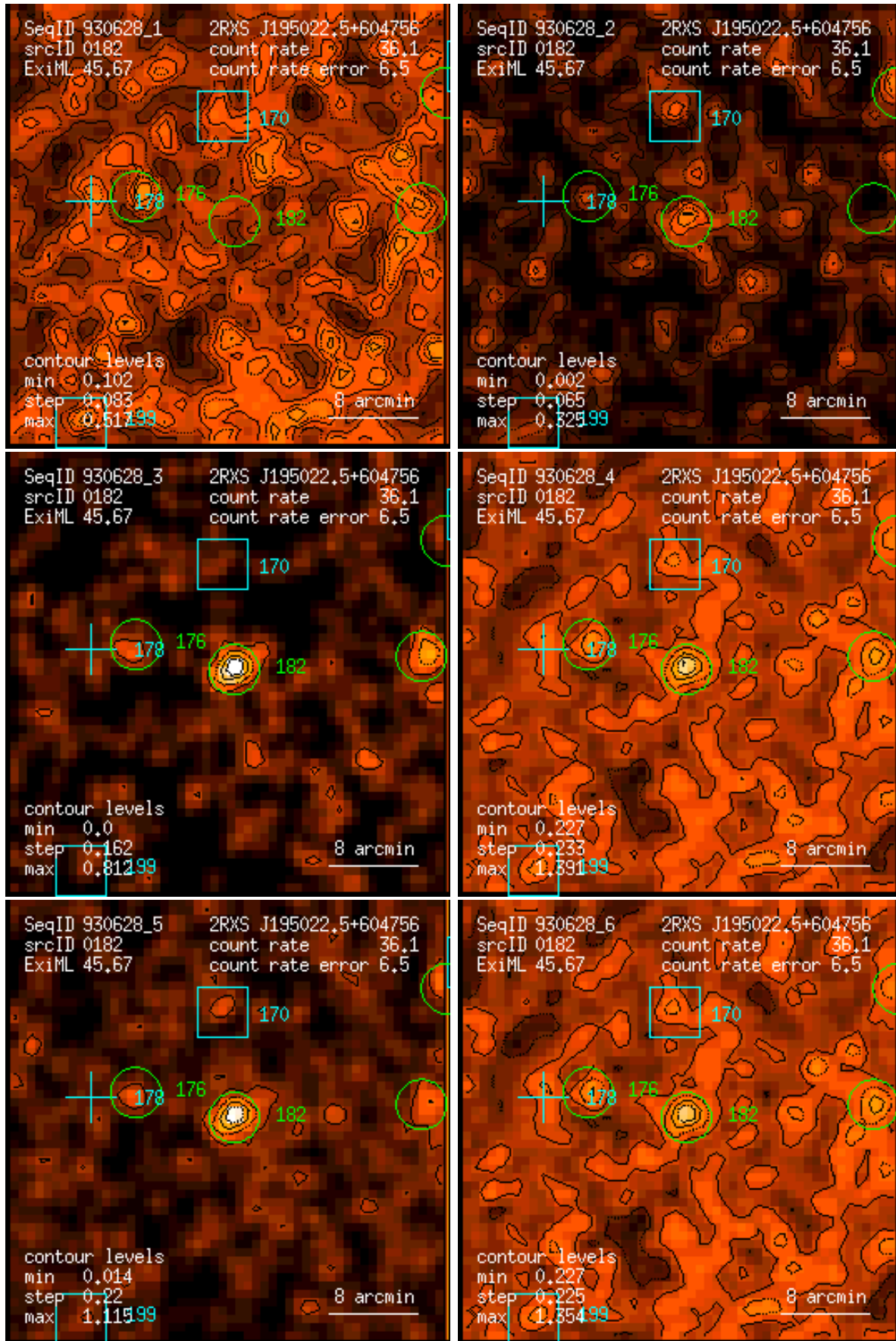
Figure 182: RASS 930628: detection 0182: band rate images, Gaussian filter: (1) PSPC channels 11 – 41, (2) 52 – 90, (3) 91 – 201, (4) 11 – 235, (5) 52 – 201, (6) 11 – 201. Broad band rates in counts/ks. Band rate contour levels in counts/ks/arcmin 2 .
