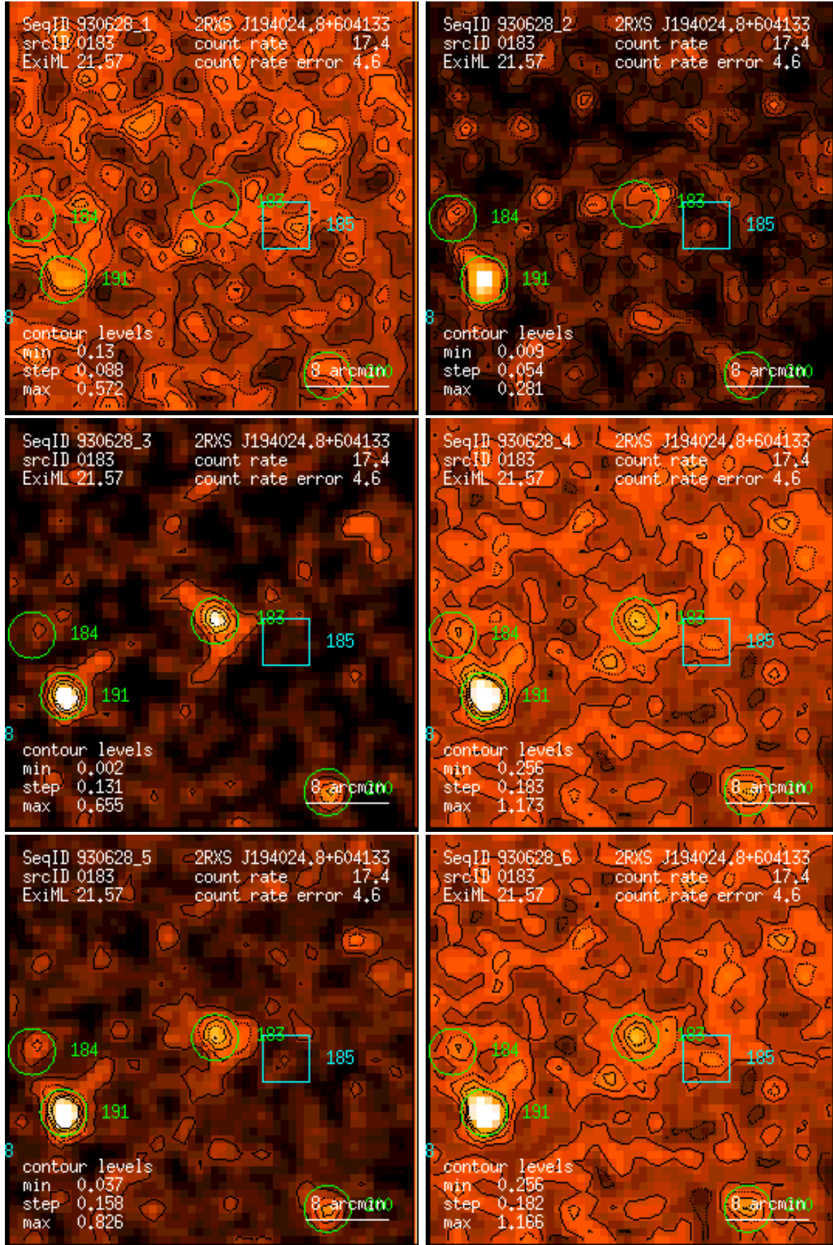
Figure 183: RASS 930628: detection 0183: band rate images, Gaussian filter: (1) PSPC channels 11 – 41, (2) 52 – 90, (3) 91 – 201, (4) 11 – 235, (5) 52 – 201, (6) 11 – 201. Broad band rates in counts/ks. Band rate contour levels in counts/ks/arcmin 2 .
