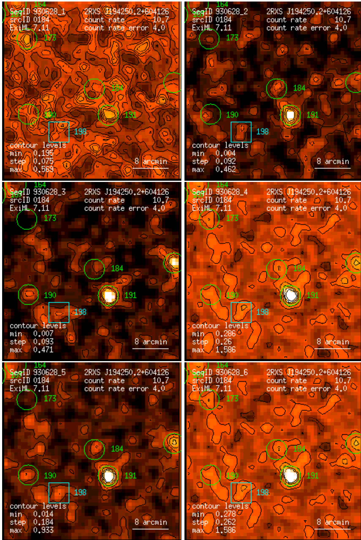
Figure 184: RASS 930628: detection 0184: band rate images, Gaussian filter: (1) PSPC channels 11 – 41, (2) 52 – 90, (3) 91 – 201, (4) 11 – 235, (5) 52 – 201, (6) 11 – 201. Broad band rates in counts/ks. Band rate contour levels in counts/ks/arcmin 2 .
