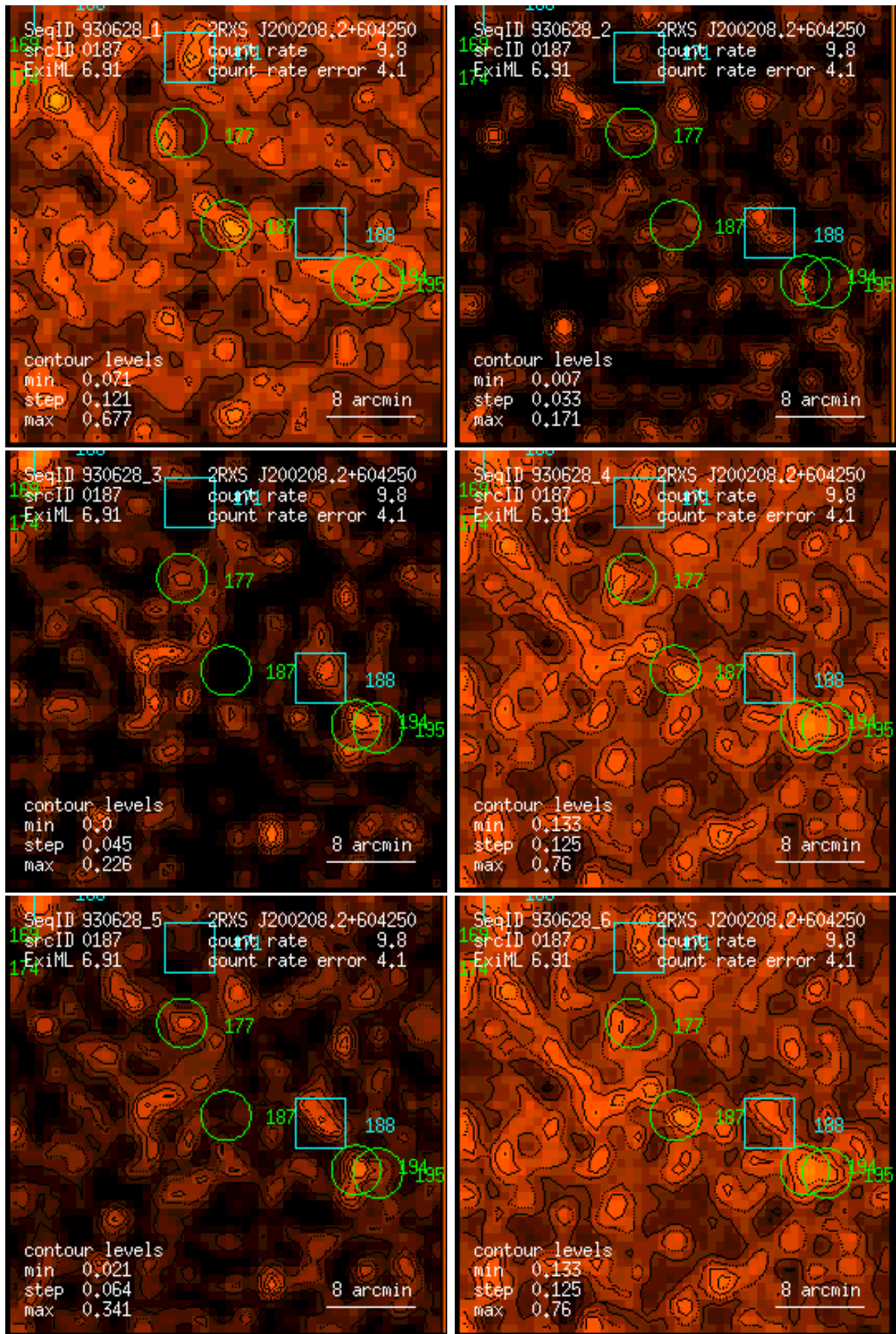
Figure 187: RASS 930628: detection 0187: band rate images, Gaussian filter: (1) PSPC channels 11 – 41, (2) 52 – 90, (3) 91 – 201, (4) 11 – 235, (5) 52 – 201, (6) 11 – 201. Broad band rates in counts/ks. Band rate contour levels in counts/ks/arcmin 2 .
