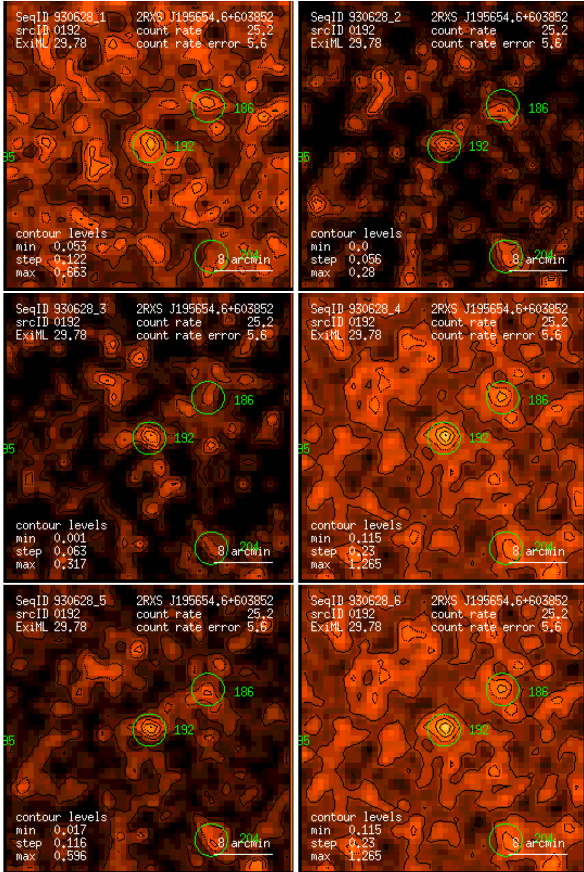
Figure 192: RASS 930628: detection 0192: band rate images, Gaussian filter: (1) PSPC channels 11 – 41, (2) 52 – 90, (3) 91 – 201, (4) 11 – 235, (5) 52 – 201, (6) 11 – 201. Broad band rates in counts/ks. Band rate contour levels in counts/ks/arcmin 2 .
