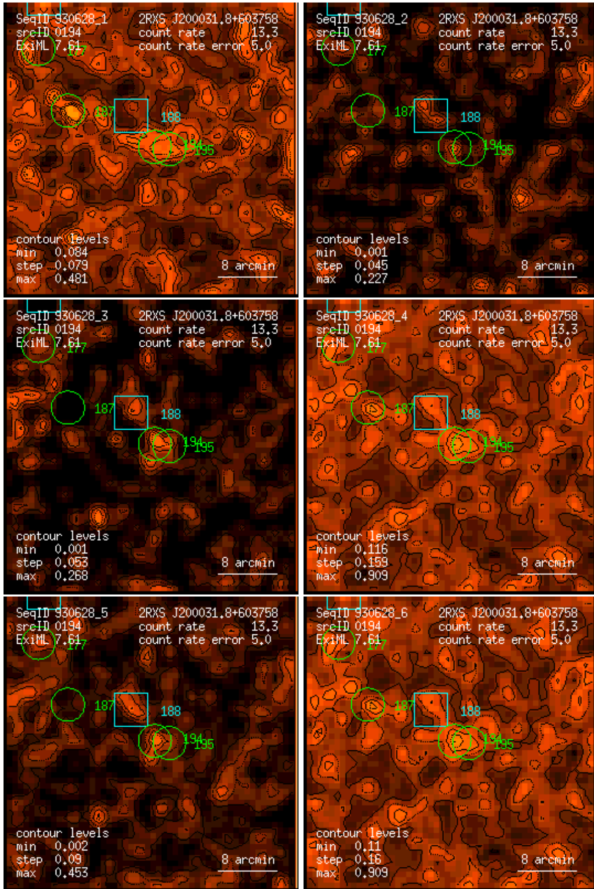
Figure 194: RASS 930628: detection 0194: band rate images, Gaussian filter: (1) PSPC channels 11 – 41, (2) 52 – 90, (3) 91 – 201, (4) 11 – 235, (5) 52 – 201, (6) 11 – 201. Broad band rates in counts/ks. Band rate contour levels in counts/ks/arcmin 2 .
