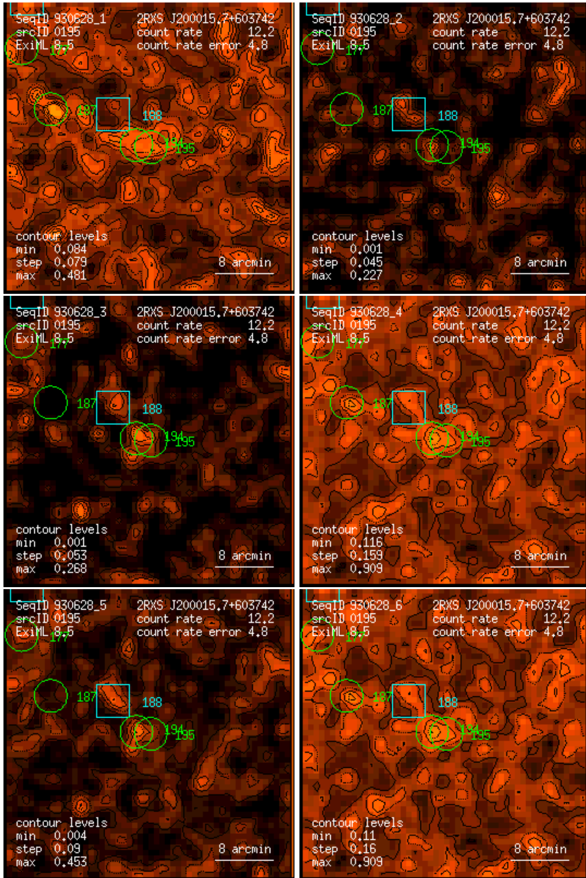
Figure 195: RASS 930628: detection 0195: band rate images, Gaussian filter: (1) PSPC channels 11 – 41, (2) 52 – 90, (3) 91 – 201, (4) 11 – 235, (5) 52 – 201, (6) 11 – 201. Broad band rates in counts/ks. Band rate contour levels in counts/ks/arcmin 2 .
