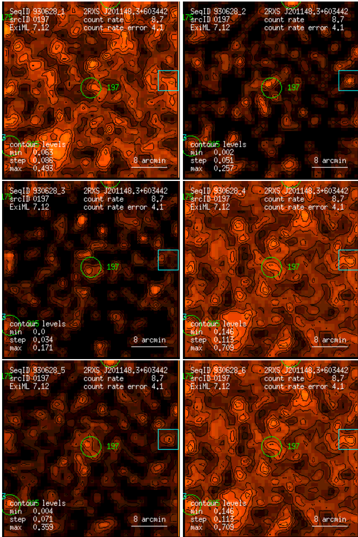
Figure 197: RASS 930628: detection 0197: band rate images, Gaussian filter: (1) PSPC channels 11 – 41, (2) 52 – 90, (3) 91 – 201, (4) 11 – 235, (5) 52 – 201, (6) 11 – 201. Broad band rates in counts/ks. Band rate contour levels in counts/ks/arcmin 2 .
