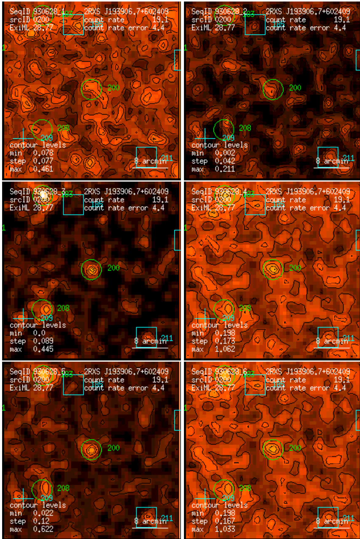
Figure 200: RASS 930628: detection 0200: band rate images, Gaussian filter: (1) PSPC channels 11 – 41, (2) 52 – 90, (3) 91 – 201, (4) 11 – 235, (5) 52 – 201, (6) 11 – 201. Broad band rates in counts/ks. Band rate contour levels in counts/ks/arcmin 2 .
