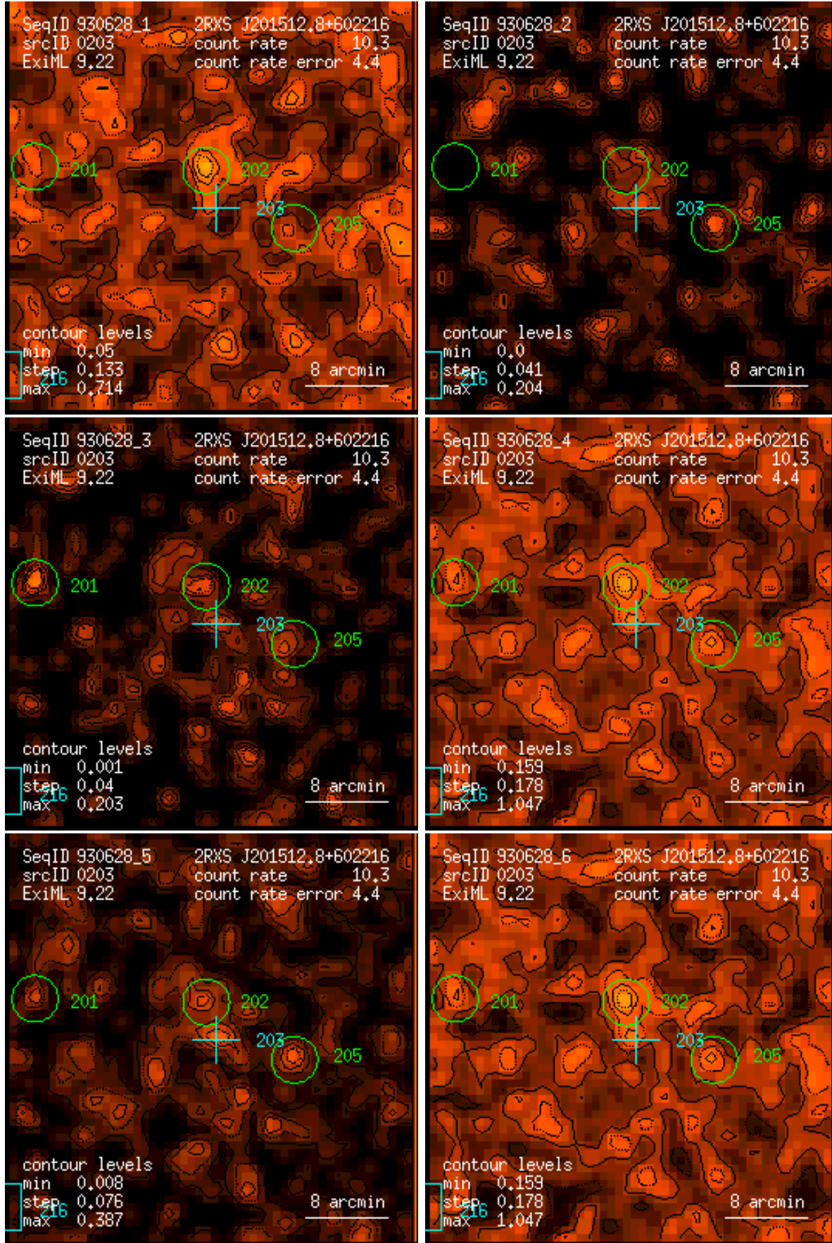
Figure 203: RASS 930628: detection 0203: band rate images, Gaussian filter: (1) PSPC channels 11 – 41, (2) 52 – 90, (3) 91 – 201, (4) 11 – 235, (5) 52 – 201, (6) 11 – 201. Broad band rates in counts/ks. Band rate contour levels in counts/ks/arcmin 2 .
