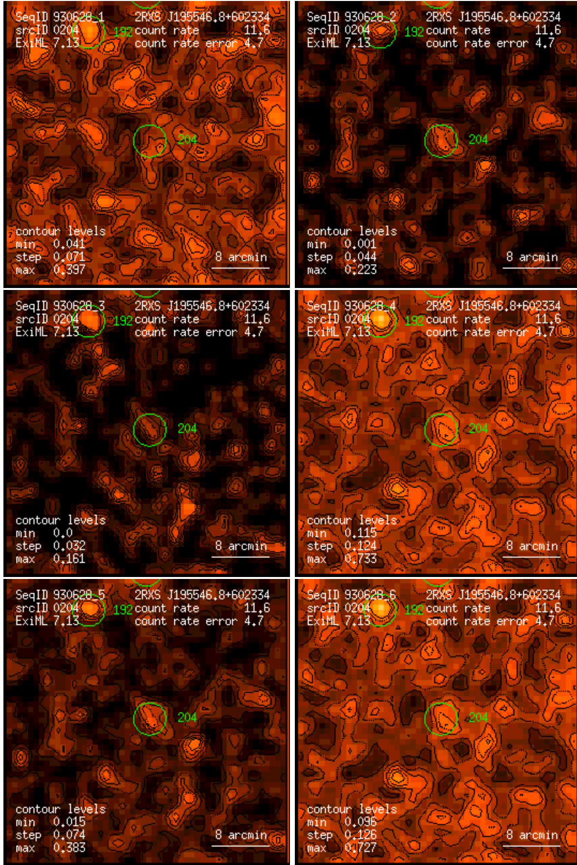
Figure 204: RASS 930628: detection 0204: band rate images, Gaussian filter: (1) PSPC channels 11 – 41, (2) 52 – 90, (3) 91 – 201, (4) 11 – 235, (5) 52 – 201, (6) 11 – 201. Broad band rates in counts/ks. Band rate contour levels in counts/ks/arcmin 2 .
