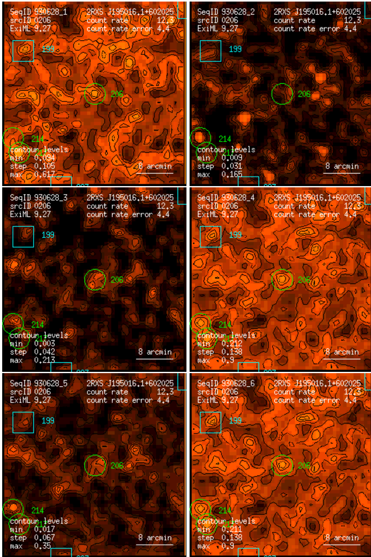
Figure 206: RASS 930628: detection 0206: band rate images, Gaussian filter: (1) PSPC channels 11 – 41, (2) 52 – 90, (3) 91 – 201, (4) 11 – 235, (5) 52 – 201, (6) 11 – 201. Broad band rates in counts/ks. Band rate contour levels in counts/ks/arcmin 2 .
