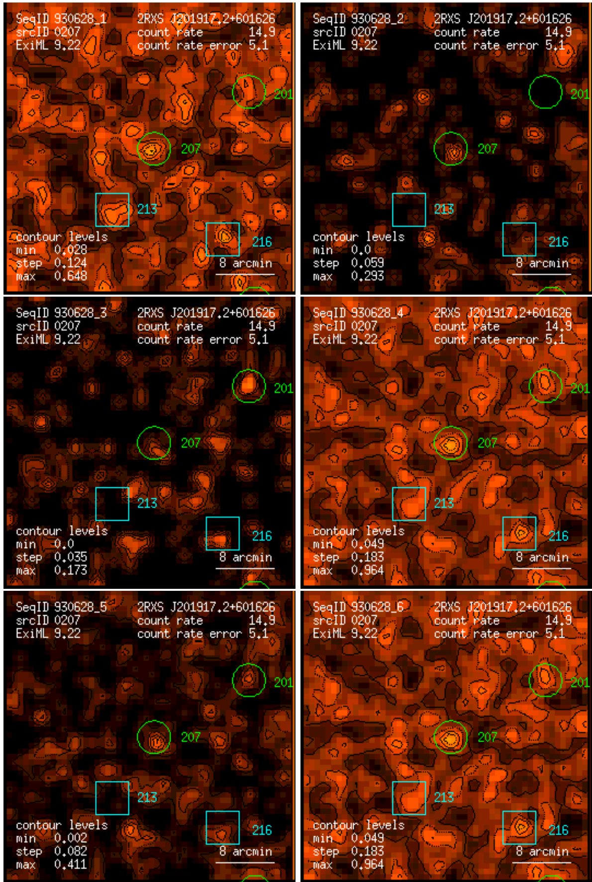
Figure 207: RASS 930628: detection 0207: band rate images, Gaussian filter: (1) PSPC channels 11 – 41, (2) 52 – 90, (3) 91 – 201, (4) 11 – 235, (5) 52 – 201, (6) 11 – 201. Broad band rates in counts/ks. Band rate contour levels in counts/ks/arcmin 2 .
