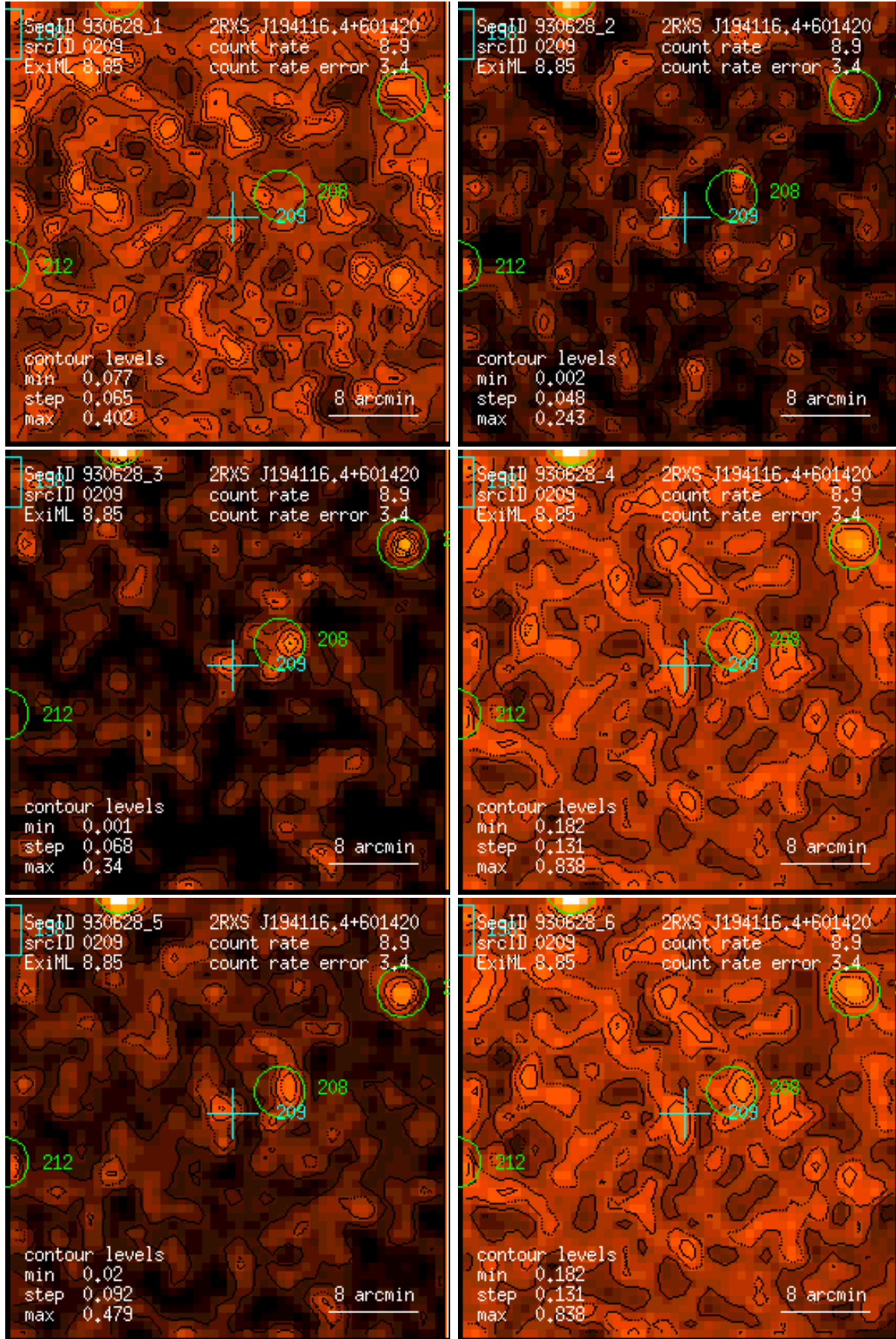
Figure 209: RASS 930628: detection 0209: band rate images, Gaussian filter: (1) PSPC channels 11 – 41, (2) 52 – 90, (3) 91 – 201, (4) 11 – 235, (5) 52 – 201, (6) 11 – 201. Broad band rates in counts/ks. Band rate contour levels in counts/ks/arcmin 2 .
