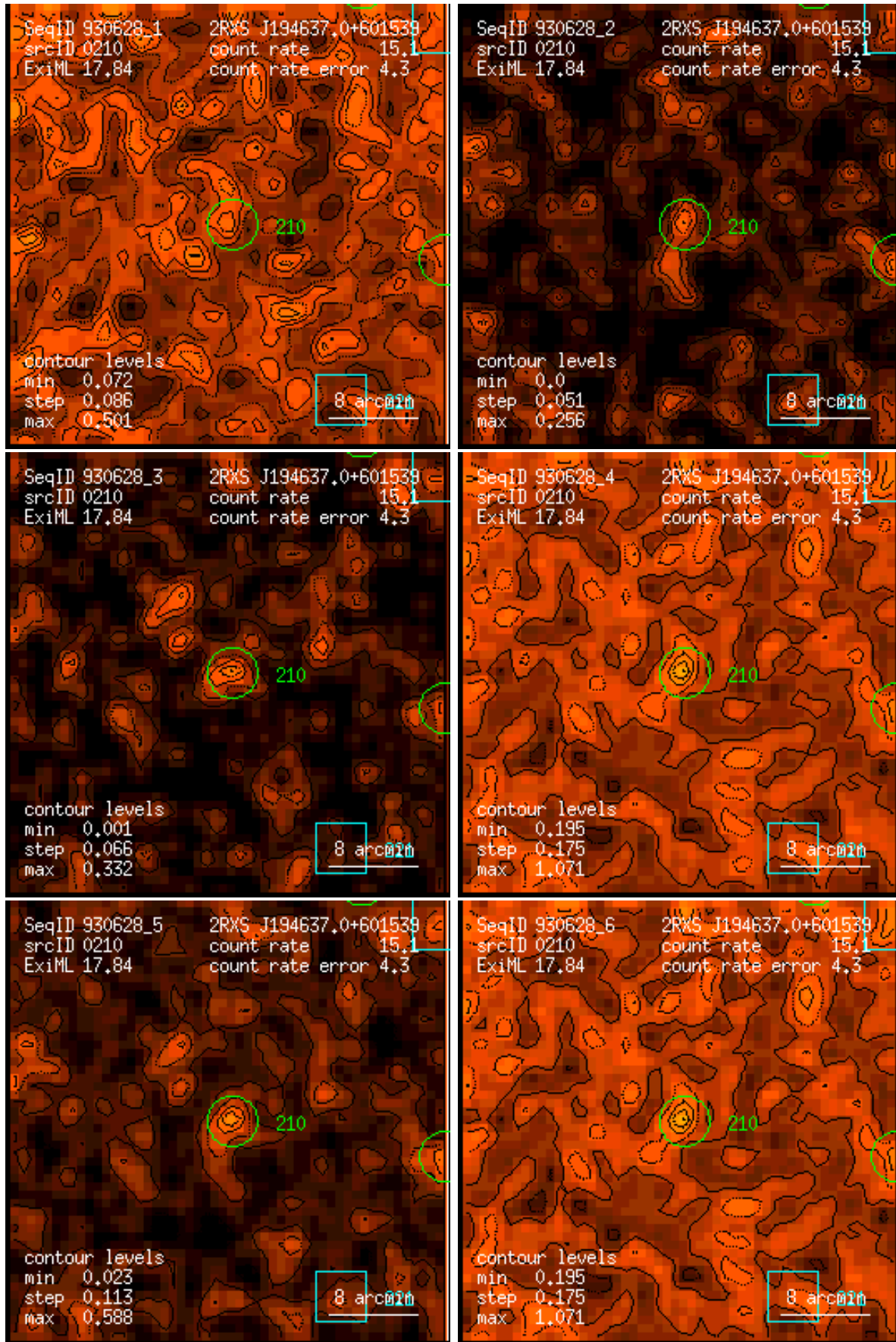
Figure 210: RASS 930628: detection 0210: band rate images, Gaussian filter: (1) PSPC channels 11 – 41, (2) 52 – 90, (3) 91 – 201, (4) 11 – 235, (5) 52 – 201, (6) 11 – 201. Broad band rates in counts/ks. Band rate contour levels in counts/ks/arcmin 2 .
