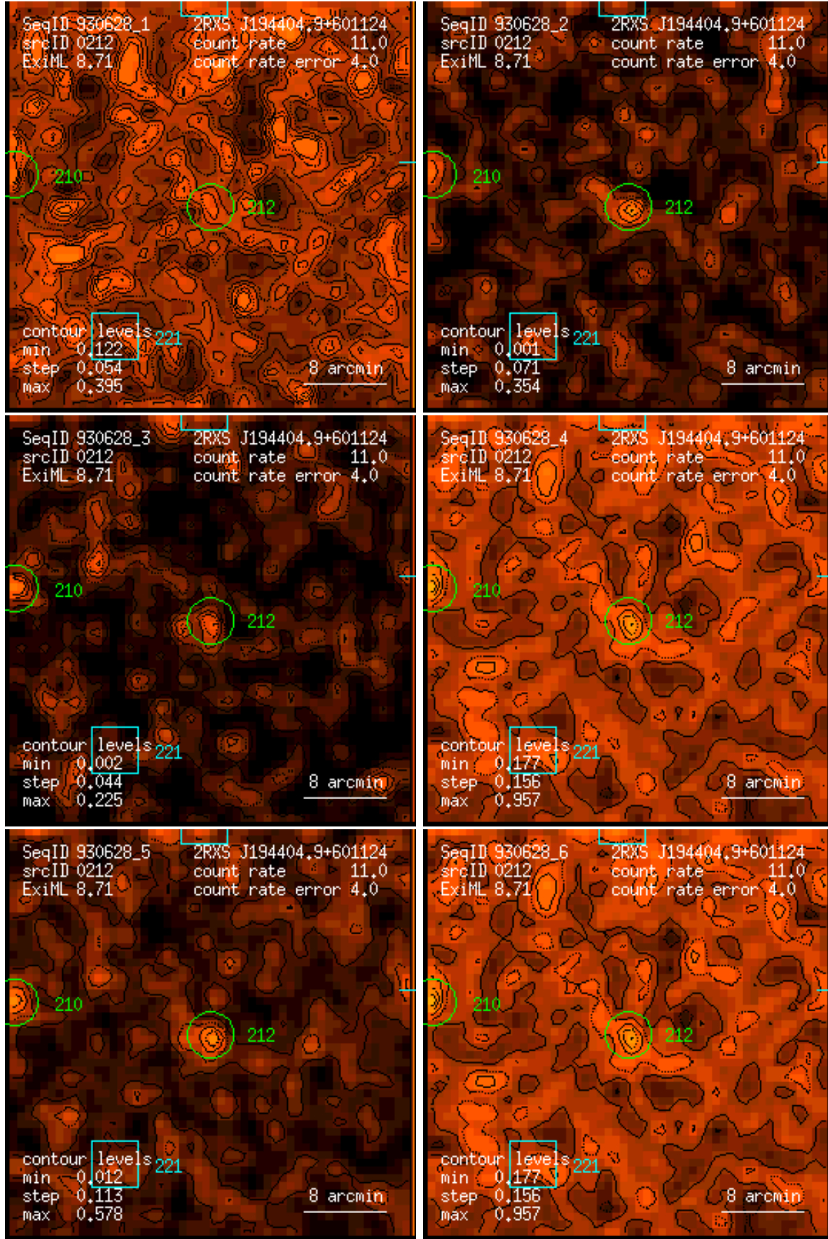
Figure 212: RASS 930628: detection 0212: band rate images, Gaussian filter: (1) PSPC channels 11 – 41, (2) 52 – 90, (3) 91 – 201, (4) 11 – 235, (5) 52 – 201, (6) 11 – 201. Broad band rates in counts/ks. Band rate contour levels in counts/ks/arcmin 2 .
