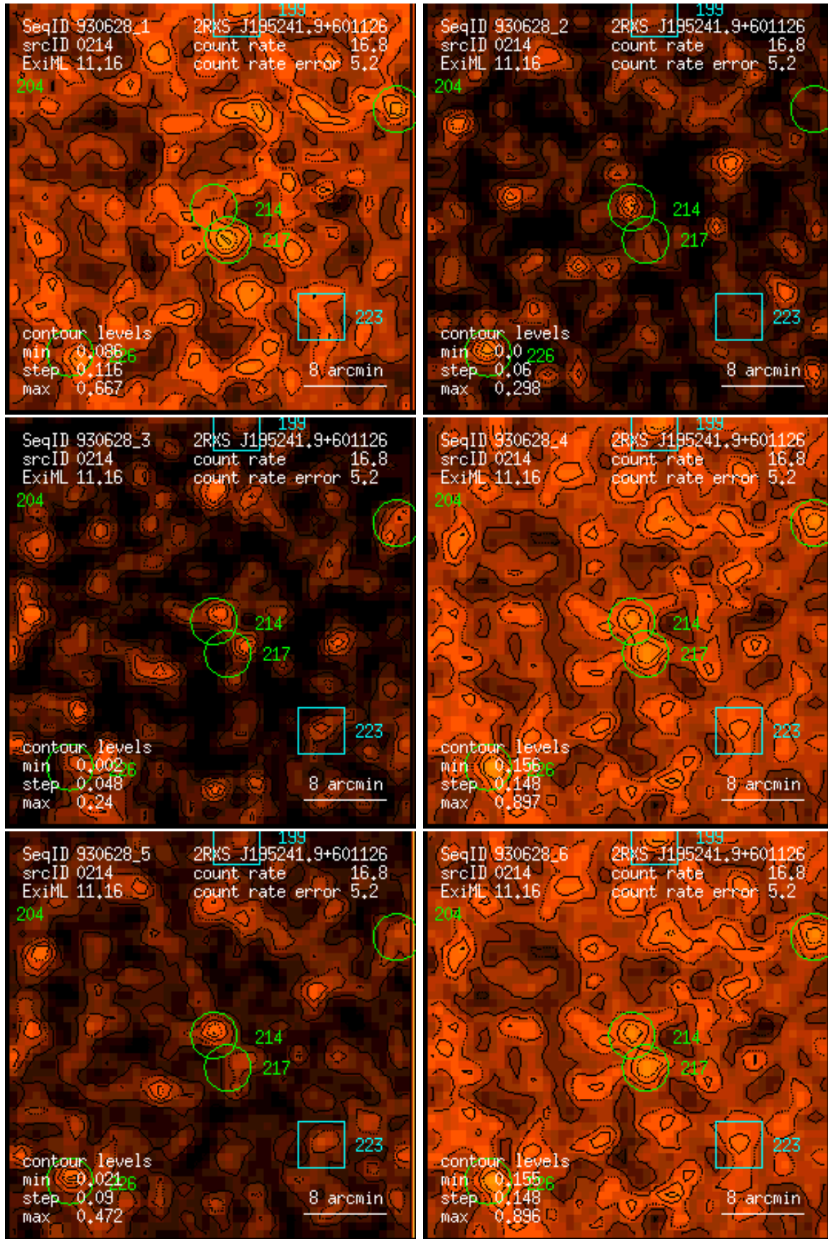
Figure 214: RASS 930628: detection 0214: band rate images, Gaussian filter: (1) PSPC channels 11 – 41, (2) 52 – 90, (3) 91 – 201, (4) 11 – 235, (5) 52 – 201, (6) 11 – 201. Broad band rates in counts/ks. Band rate contour levels in counts/ks/arcmin 2 .
