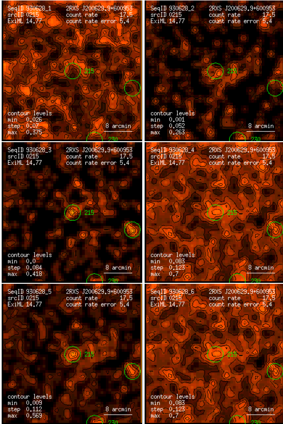
Figure 215: RASS 930628: detection 0215: band rate images, Gaussian filter: (1) PSPC channels 11 – 41, (2) 52 – 90, (3) 91 – 201, (4) 11 – 235, (5) 52 – 201, (6) 11 – 201. Broad band rates in counts/ks. Band rate contour levels in counts/ks/arcmin 2 .
