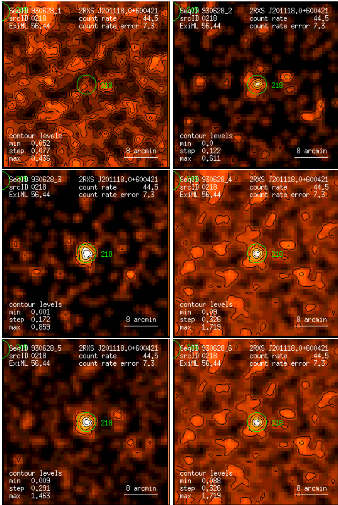
Figure 218: RASS 930628: detection 0218: band rate images, Gaussian filter: (1) PSPC channels 11 – 41, (2) 52 – 90, (3) 91 – 201, (4) 11 – 235, (5) 52 – 201, (6) 11 – 201. Broad band rates in counts/ks. Band rate contour levels in counts/ks/arcmin 2 .
