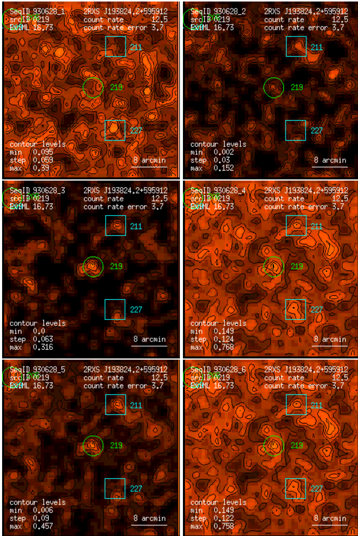
Figure 219: RASS 930628: detection 0219: band rate images, Gaussian filter: (1) PSPC channels 11 – 41, (2) 52 – 90, (3) 91 – 201, (4) 11 – 235, (5) 52 – 201, (6) 11 – 201. Broad band rates in counts/ks. Band rate contour levels in counts/ks/arcmin 2 .
