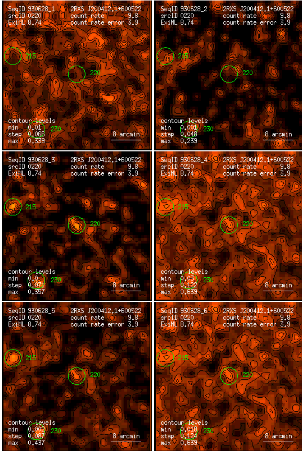
Figure 220: RASS 930628: detection 0220: band rate images, Gaussian filter: (1) PSPC channels 11 – 41, (2) 52 – 90, (3) 91 – 201, (4) 11 – 235, (5) 52 – 201, (6) 11 – 201. Broad band rates in counts/ks. Band rate contour levels in counts/ks/arcmin 2 .
