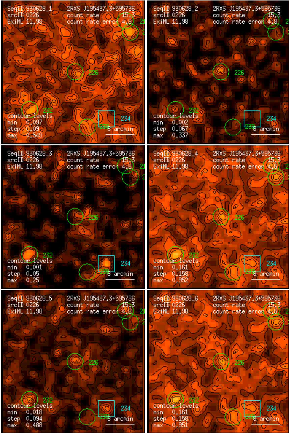
Figure 226: RASS 930628: detection 0226: band rate images, Gaussian filter: (1) PSPC channels 11 – 41, (2) 52 – 90, (3) 91 – 201, (4) 11 – 235, (5) 52 – 201, (6) 11 – 201. Broad band rates in counts/ks. Band rate contour levels in counts/ks/arcmin 2 .
