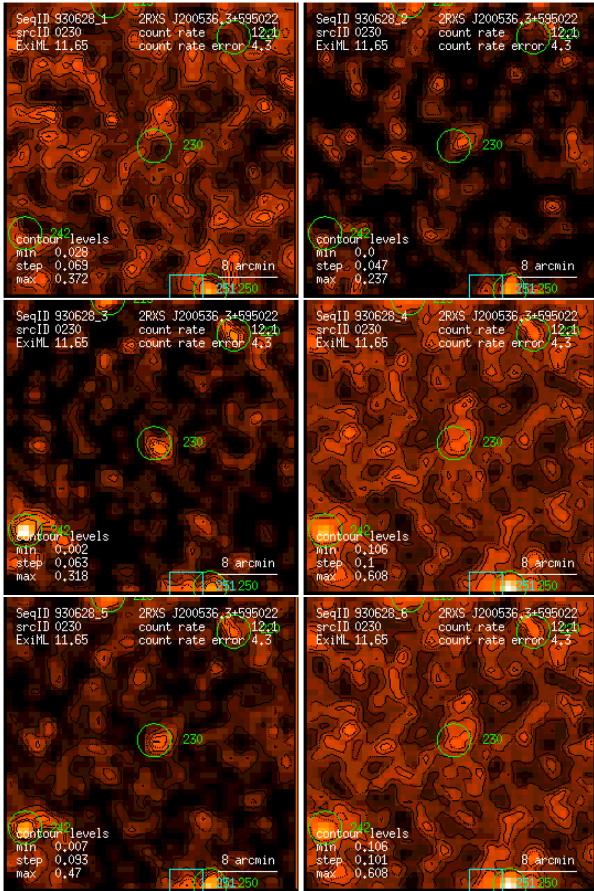
Figure 230: RASS 930628: detection 0230: band rate images, Gaussian filter: (1) PSPC channels 11 – 41, (2) 52 – 90, (3) 91 – 201, (4) 11 – 235, (5) 52 – 201, (6) 11 – 201. Broad band rates in counts/ks. Band rate contour levels in counts/ks/arcmin 2 .
