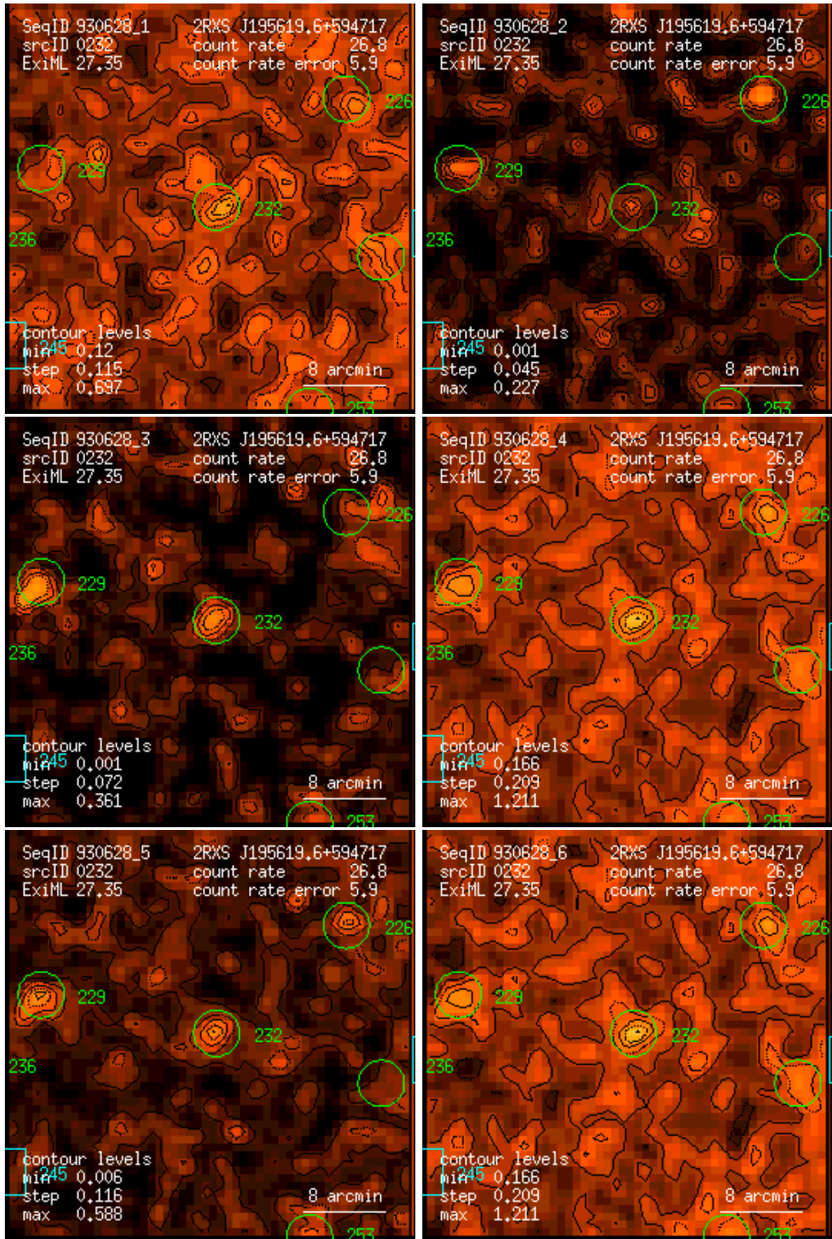
Figure 232: RASS 930628: detection 0232: band rate images, Gaussian filter: (1) PSPC channels 11 – 41, (2) 52 – 90, (3) 91 – 201, (4) 11 – 235, (5) 52 – 201, (6) 11 – 201. Broad band rates in counts/ks. Band rate contour levels in counts/ks/arcmin 2 .
