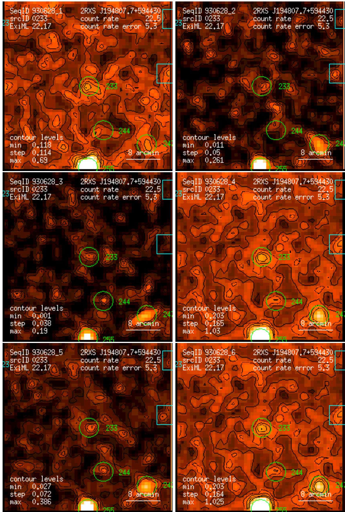
Figure 233: RASS 930628: detection 0233: band rate images, Gaussian filter: (1) PSPC channels 11 – 41, (2) 52 – 90, (3) 91 – 201, (4) 11 – 235, (5) 52 – 201, (6) 11 – 201. Broad band rates in counts/ks. Band rate contour levels in counts/ks/arcmin 2 .
