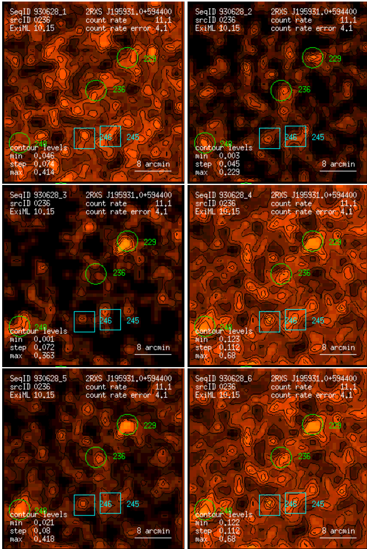
Figure 236: RASS 930628: detection 0236: band rate images, Gaussian filter: (1) PSPC channels 11 – 41, (2) 52 – 90, (3) 91 – 201, (4) 11 – 235, (5) 52 – 201, (6) 11 – 201. Broad band rates in counts/ks. Band rate contour levels in counts/ks/arcmin 2 .
